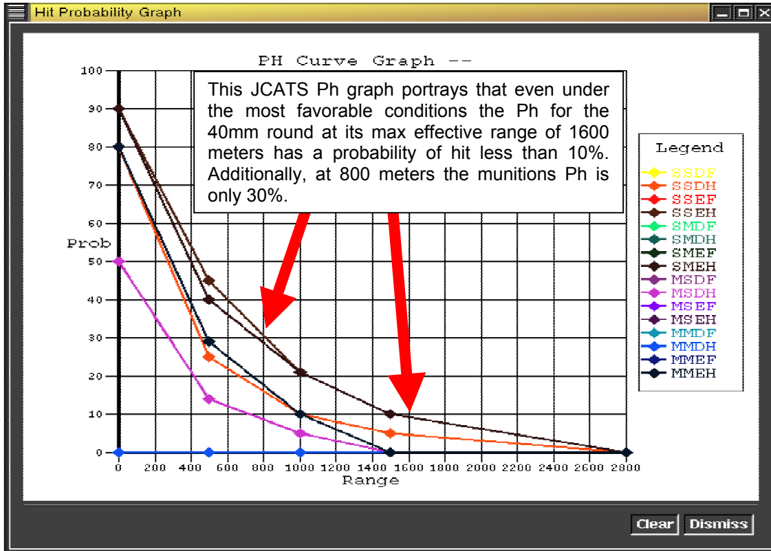
Figure 23. JCATS Ph Curve Data for 40mm Muniton
