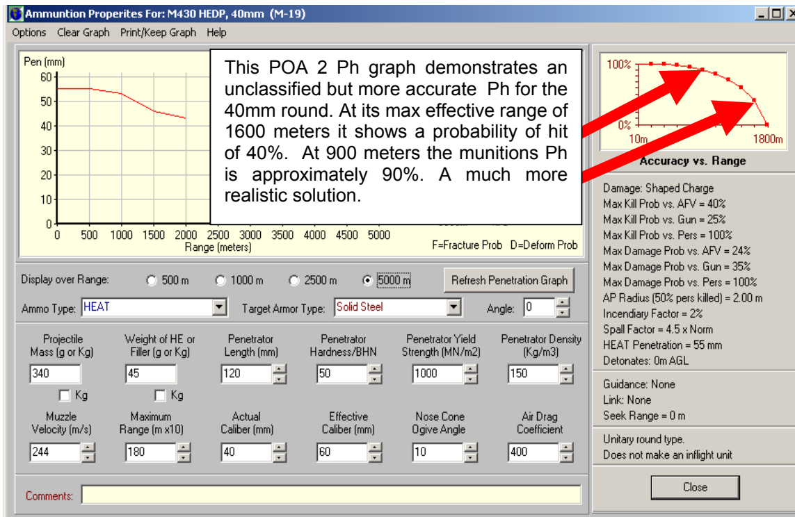
Figure 24. POA2 Ammunition Properties for 40mm Muniton
