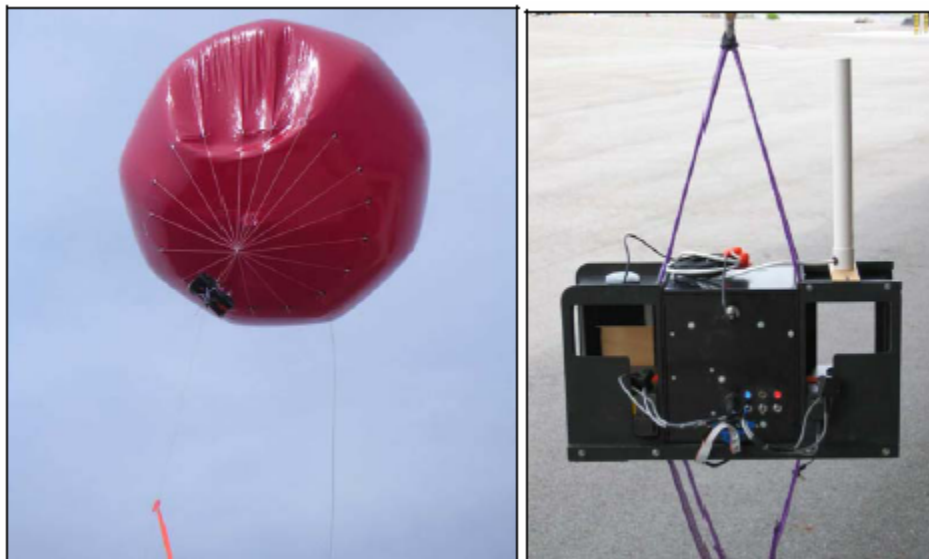
Figure 10. Balloon and Payload
