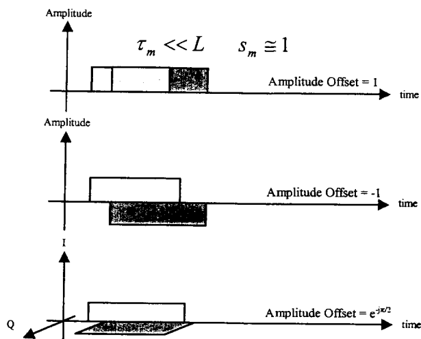
Figure 7 Visualizing Highly Overlapped STORM Signals
