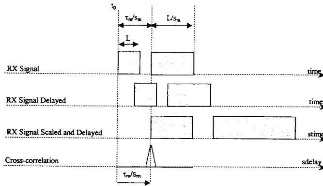
Figure 8 Synchronous Reception
