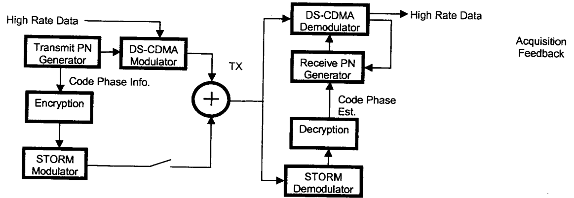
Figure 13 STORM Assisted DS-CDMA Acquisition
