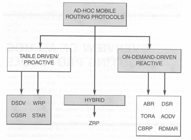
Figure 12. Ad hoc Routing Protocols (From [2])
