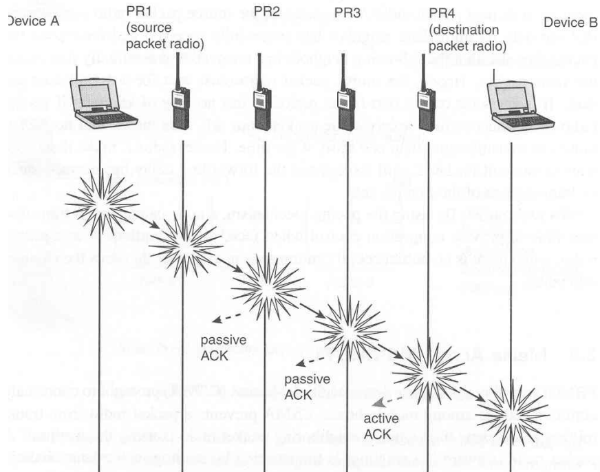
Figure 2. Passive and Active Acknowledgements in PRNET (From [2]).
