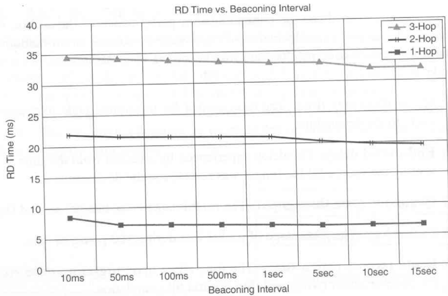
Figure 20. Route discovery time vs. beaconing interval (From [2]).
