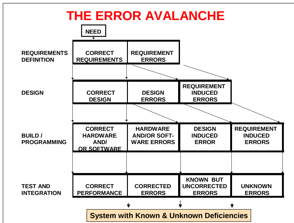
Figure 26. Requirements Instability
