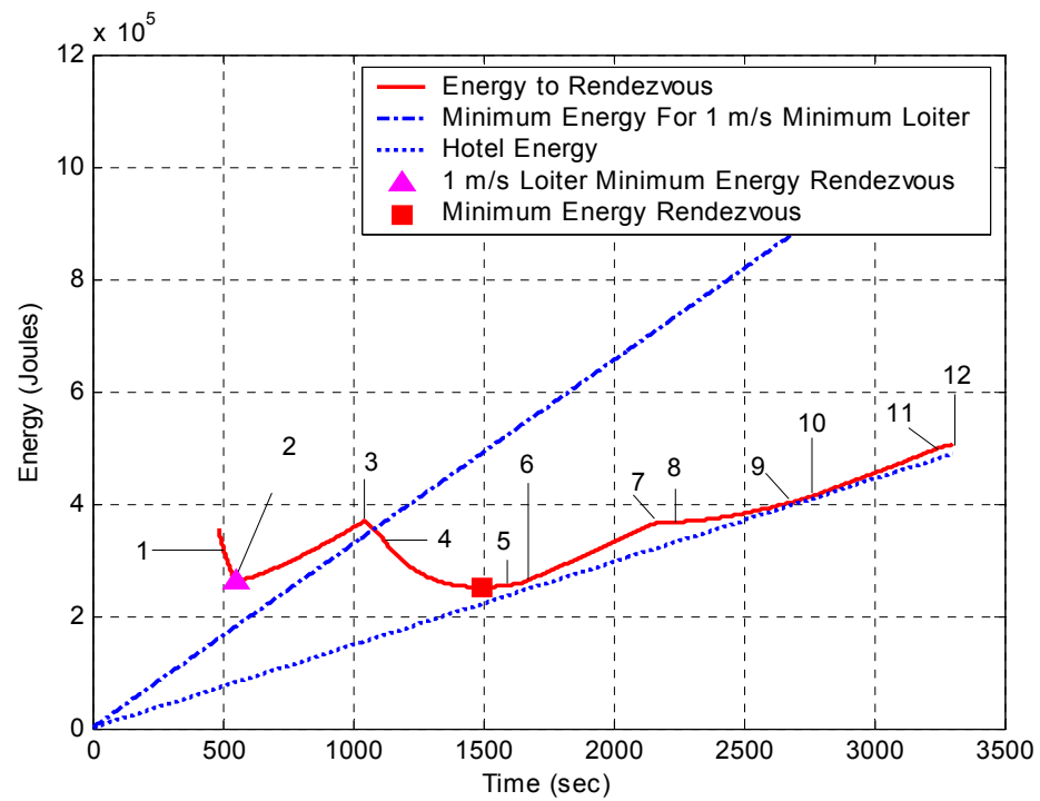
Figure 16. ARIES Rendezvous With Maneuvering Target, Waypoints Annotated
