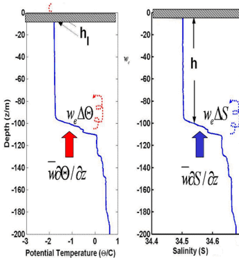
Figure 10. When ice is present all entrained heat is fluxed into the ice (Garwood, 2004).
