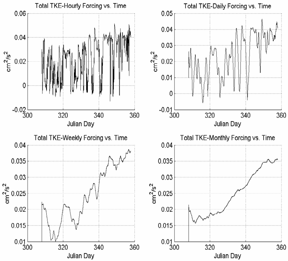
Figure 42. Western Arctic Total TKE
