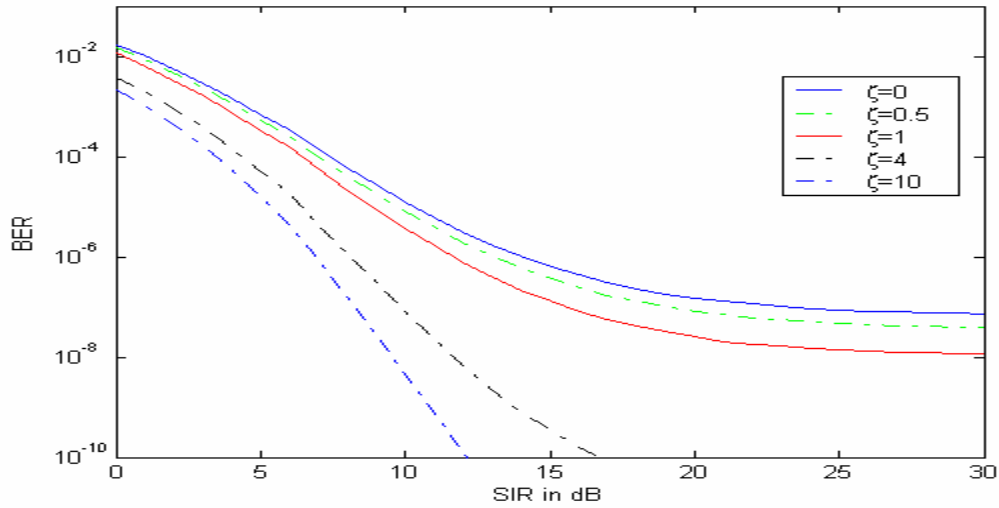
Figure 22. BPSK/QPSK with convolutional coding and SDD for r = 1/2 in a Ricean channel, with AWGN and pulsed-noise interference ( p = 0.5 ).
