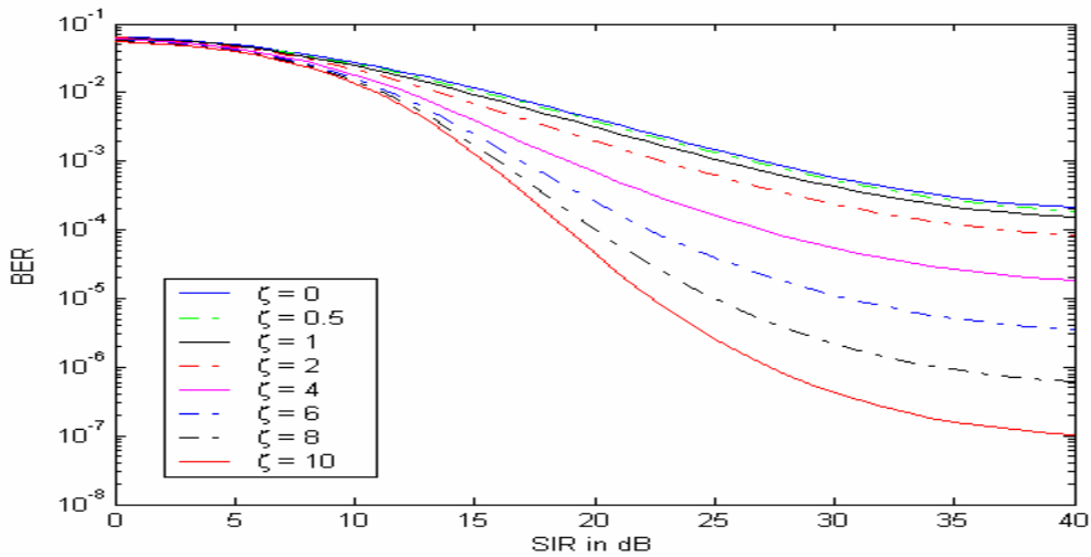
Figure 6. 16-QAM in Ricean channel with AWGN and pulsed-noise interference ( p = 0.5 ).
