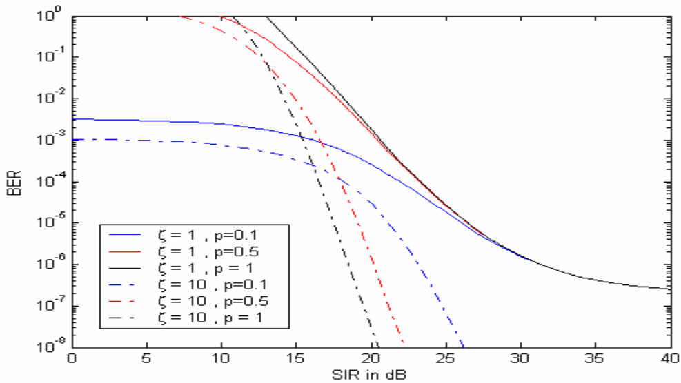
Figure 19. 64-QAM with convolutional coding and HDD with r = 2/3 in a Ricean channel with AWGN and pulsed-noise interference.
