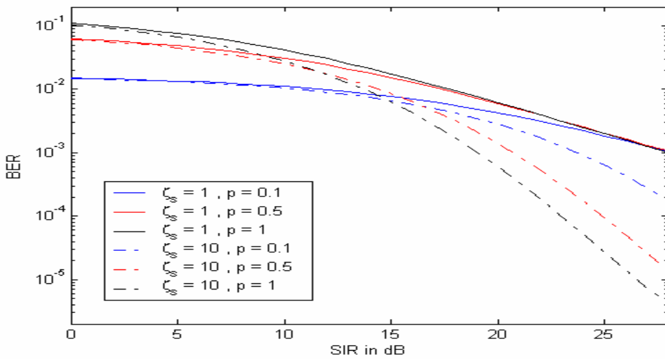
Figure 49. 64-QAM transmitted over a Ricean fading channel with Rayleigh fading pulsed-noise interference and AWGN.
