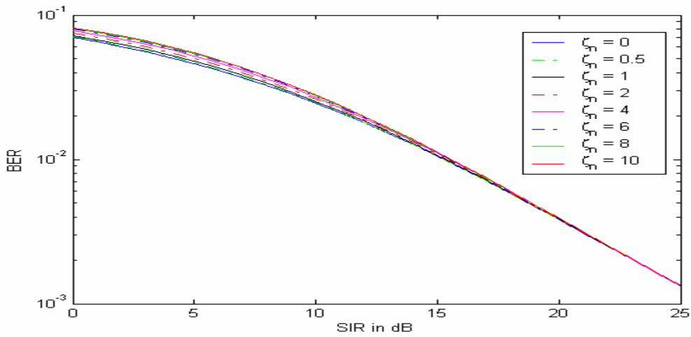
Figure 28. 16-QAM transmitted over a Rayleigh fading channel with Ricean fading pulsed-noise interference ( p = 0.5 ) and AWGN.
