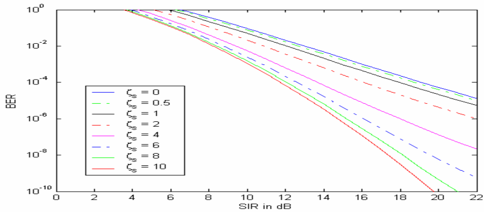
Figure 52. BPSK/QPSK with r = 3/4 convolutional coding and HDD transmitted over a Ricean fading channel with Rayleigh fading pulsed-noise interference ( p = 0.5 ) and AWGN.
