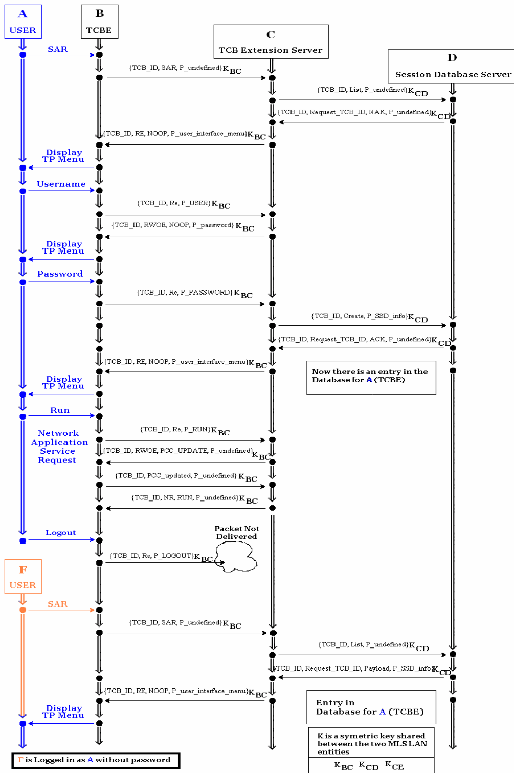
Figure 16. Interconnections of the MLS LAN Protocol Suite
