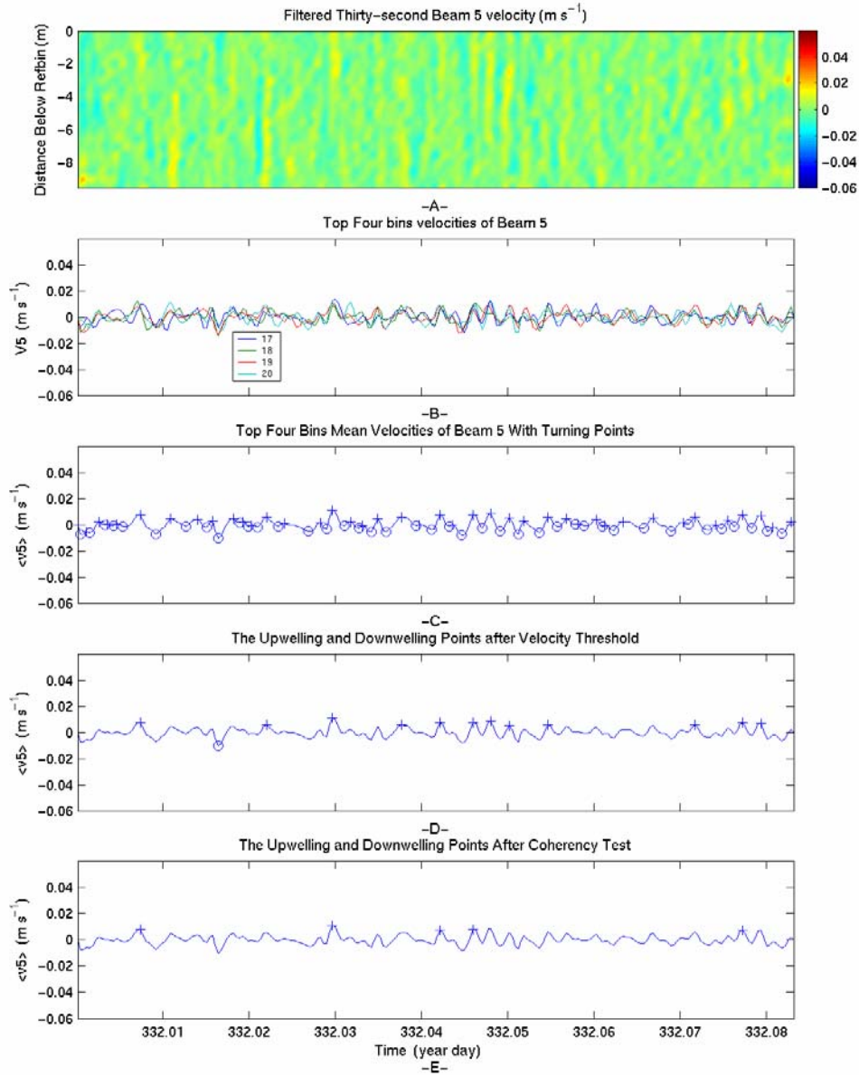
Figure 4.17 Detection of upwelling / downwelling regions of Langmuir circulations between the days 332 and 332.0833. The wind speed is \sim 1 \text{ ms}^{-1} and the wave height is \sim 0 \text{ m} . 5 upwelling regions (Panel E) were detected. This is the time period right before a storm case between the days 332.6 and 334.
