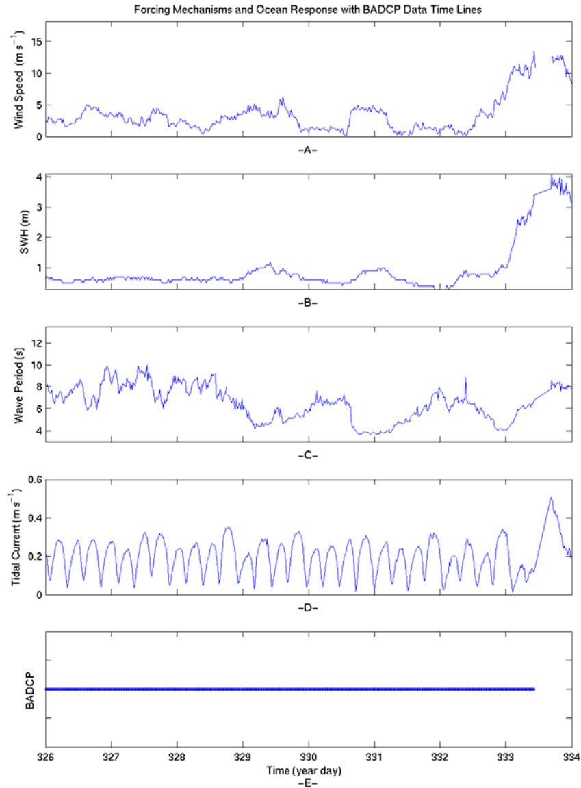
Figure 4.14 Atmospheric and oceanic forcing mechanisms with the available ADCP data in winter time between the days 326 and 334. The wind speed in Panel A is low to moderate till the day 332.3 and after this day storm system is effective. The increasing wind speed from 0 to 14 \text{ m s}^{-1} between the days 332.3 and 333.5, trigger the ocean and wave heights in Panel B increases from 0 to 4 m during the same time period which is a good case for Langmuir circulation development. The wave period is in Panel C and the tidal currents at the surface in Panel D, which are strong enough to compete with the Langmuir circulations horizontal velocities. Times of available ADCP data are in Panel E for this time period of year.
