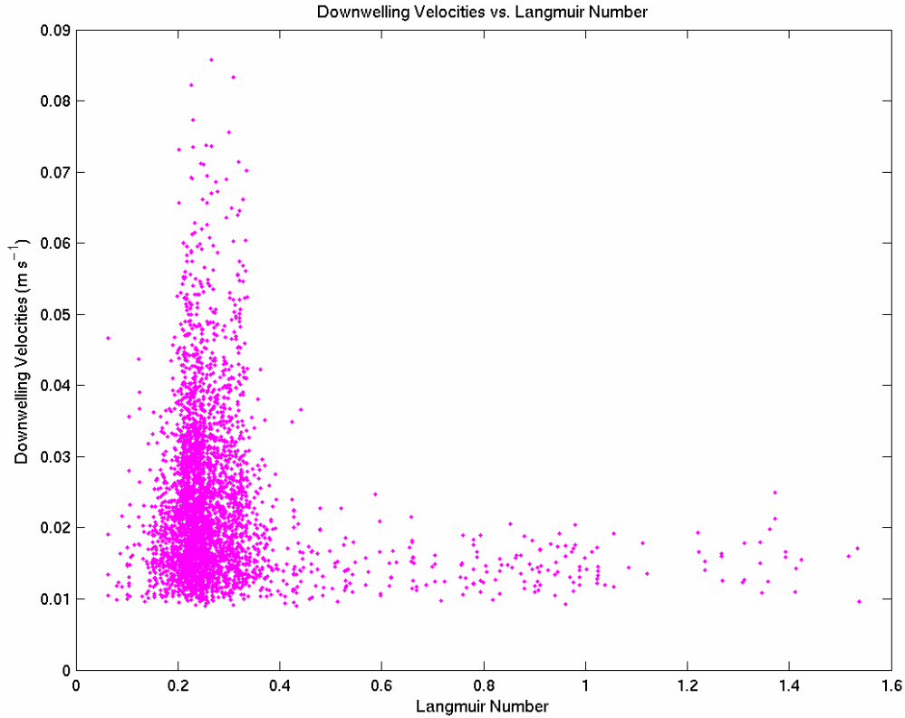
Figure 5.10 Downwelling velocities and Langmuir number relationship between the days 288 and 295.5; 314.5 and 319; 331.5 and 338.5; 344 and 360.
