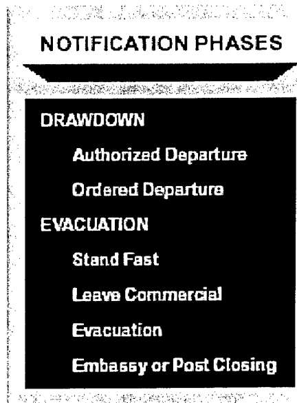
Figure 13. Notification Phases
