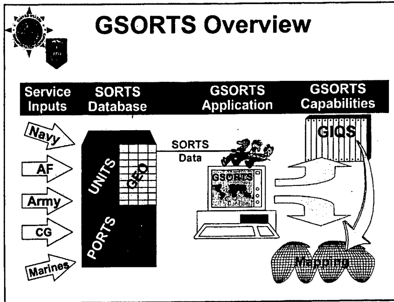
Figure 8. GSORTS Overview
