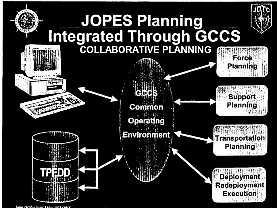
Figure 4. JOPES-GCCS Interface
