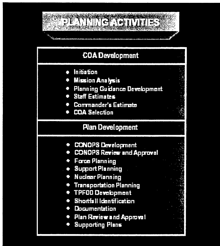
Figure III-2. Planning Activities
