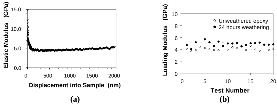
Figure 4.2.2-3. Elastic modulus measured using nanoindentation (a) as a function of penetration depth and (b) average loading modulus for unweathered coatings and after 24 hours of weathering.
