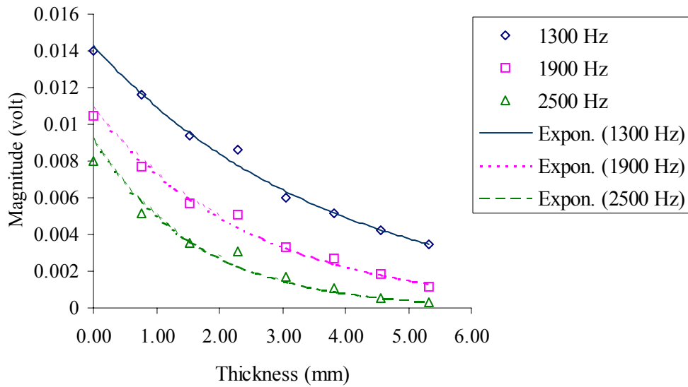
Figure 4.1.3-2. Changes in GMR signal magnitude (at three frequencies) with thickness. The sample was a multi-layered laboratory specimen.
