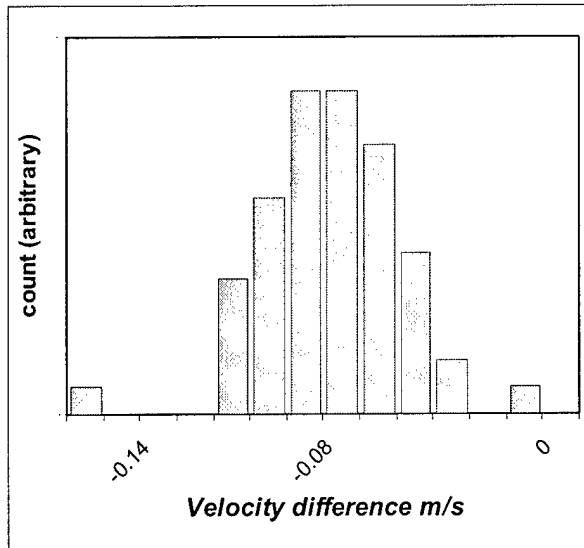
Figure 18: The histogram of LVG record.
