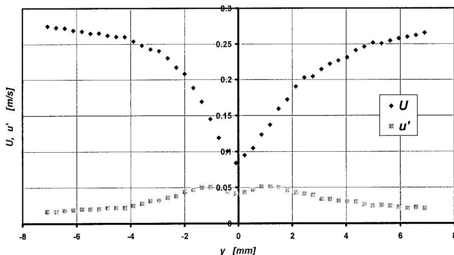
Figure 19: Mean and rms profiles of streamwise velocity in mixing layer ( U_1/U_2 = 1 )
