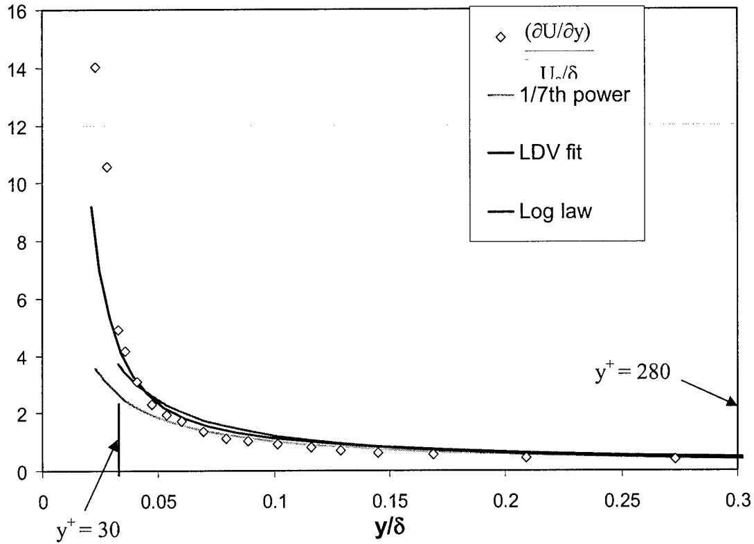
Figure 50: Near wall profile of \partial U / \partial y (TBL 2)
