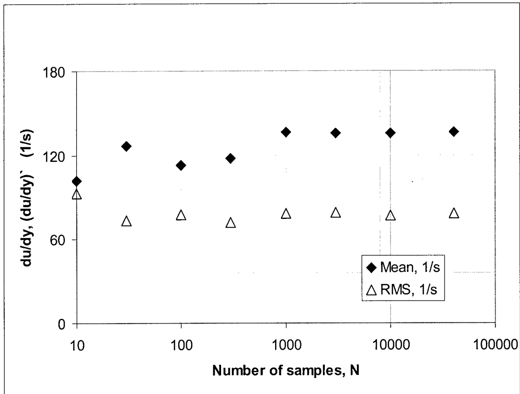
Figure 33: Effect of sampling length on mean and turbulent velocity gradient
