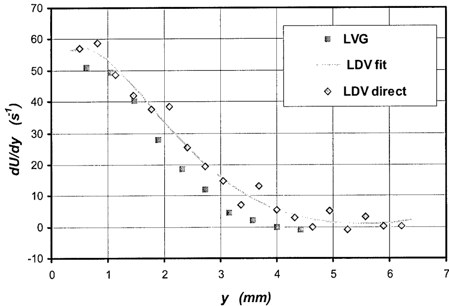
Figure 34: Comparison of velocity gradients obtained from LDV profiles and the LVG probe for BL 1
