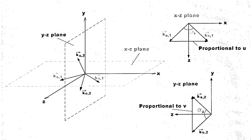
Fig. 2: Optical configuration for the vorticity probe
