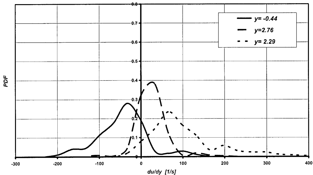
Figure 26: Probability density function of \partial u/\partial y for U_1/U_2 = 0.5
