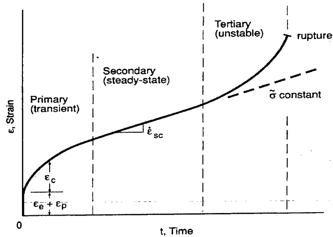
Figure 1.3: Strain vs. Time Behavior of Creep [Dowling, 1999].
