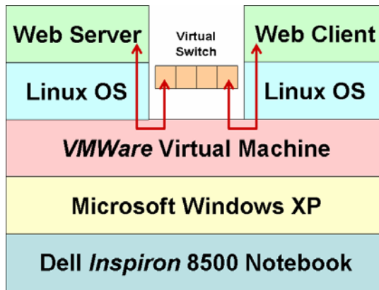
Figure 4. Virtual Network Environment (VNE).
