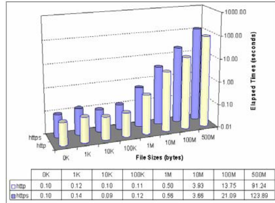
Figure 9. Client in VNE, server in PNE.
