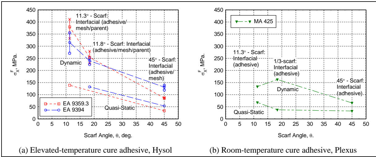
Figure 10. Axial compressive strength of scarf-repaired composite specimens under dynamic compressive load.
