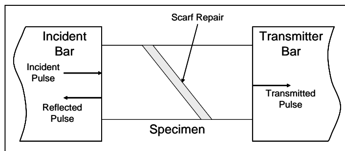
Figure 4. Hopkinson bar procedure for dynamic axial compression of scarf repair composite specimens.
