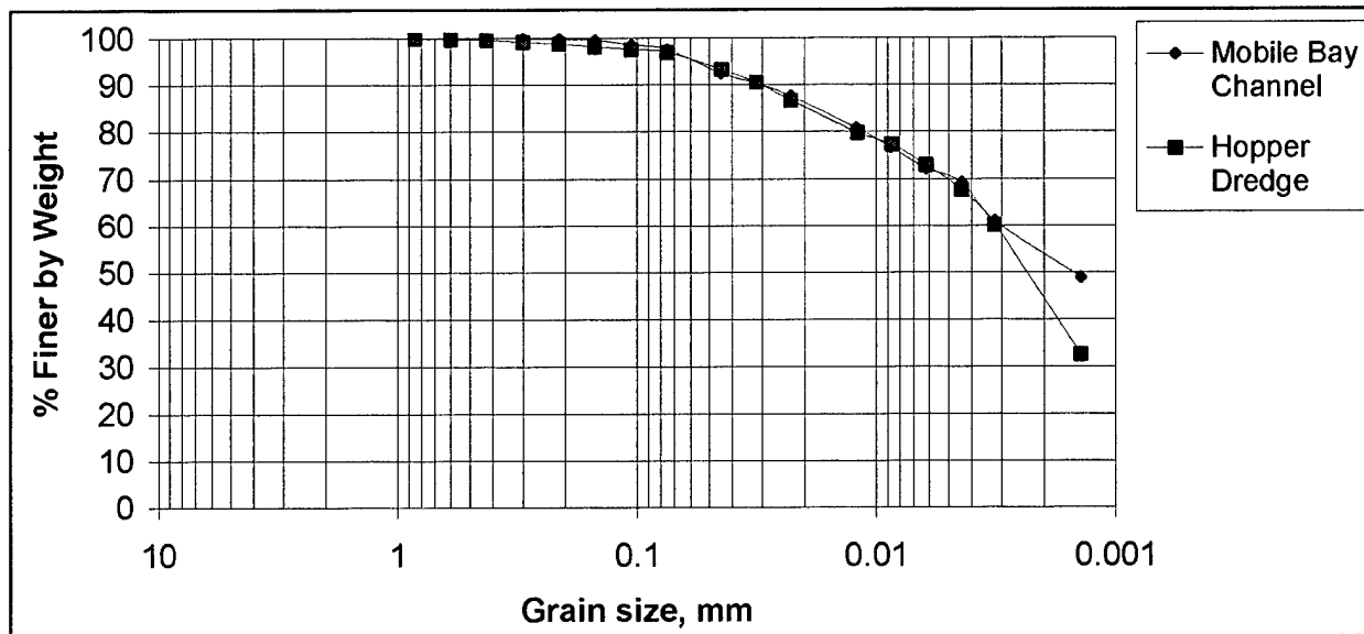
Figure 7. Cumulative grain size distribution (by weight) curves for dredged material samples taken prior to dredging (Mobile Bay Channel) and post-dredged (Hopper Dredge)
