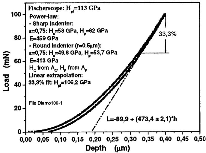
Figure 3: Example of indentation into a bulk industrial diamond with L_{max} = 100 mN. The values of hardness obtained by the linear extrapolation agree reasonably well with that from Fischerscope but the power law fit yields too low values.
