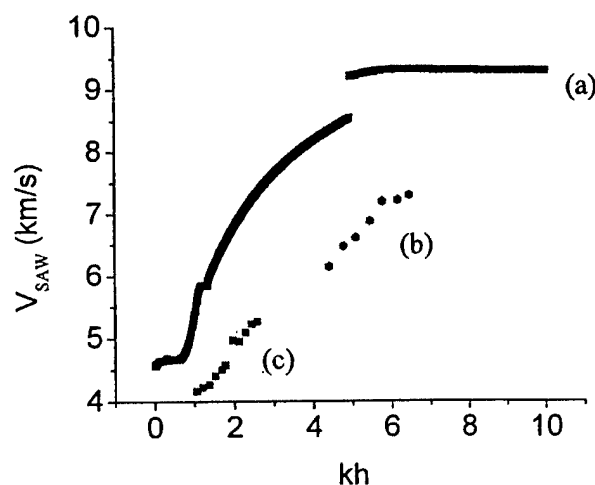
FIG. 12. Theoretical SAW dispersion of 500 nm cBN film on Si(111) calculated for direction [1\bar{1}1] (a); and experimental data (Ref. 11) for 277 nm cBN film (b); and 123 nm cBN film (c).
