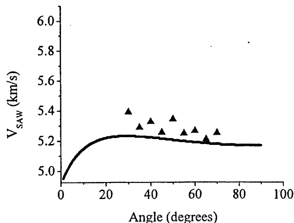
FIG. 9. Theoretical SAW dispersion curve for cBN film (16 nm cBN/15 nm hBN) on Si(001) calculated for [100] direction, and compared with experimental data (triangles).
