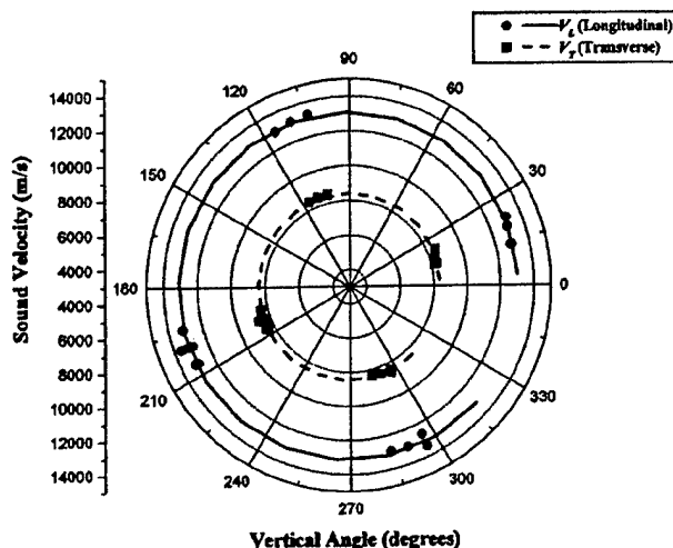
FIG. 2. Experimental azimuth dependence of longitudinal (solid circles) and shear velocities (solid squares) in c -BC 2 N. Thick lines are linear fits to present data.
