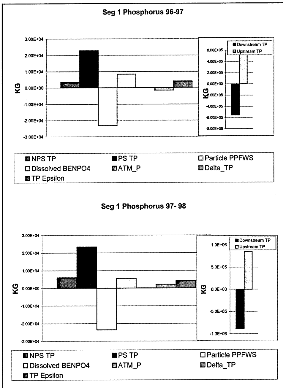
Figure 10-6. TP budget by segments for both simulation years (Sheet 1 of 6)
