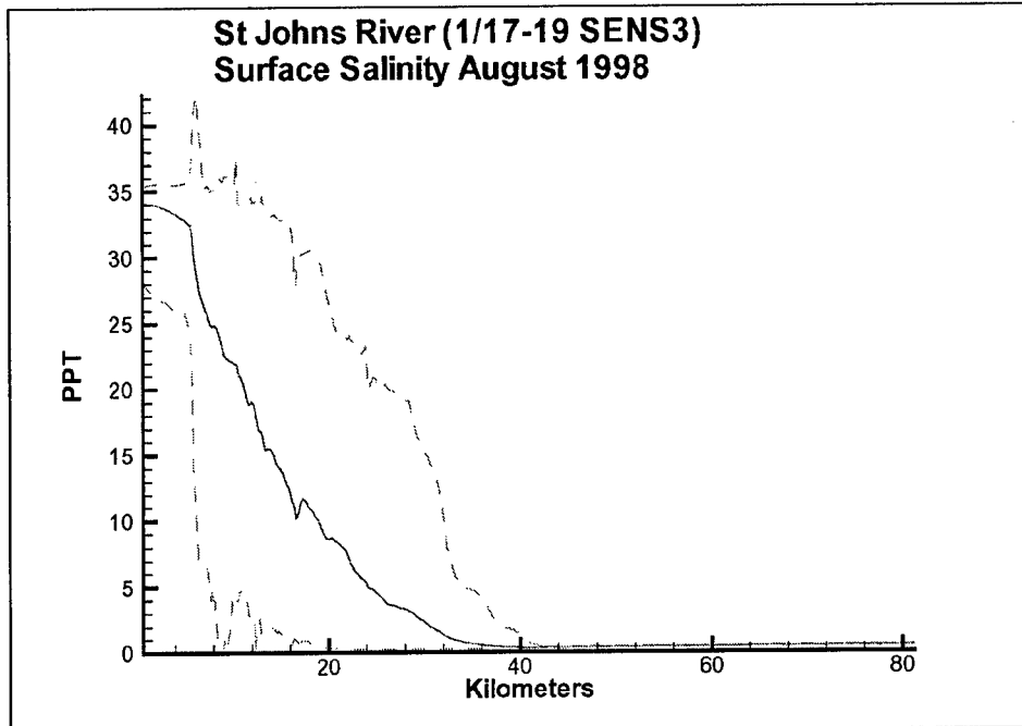
Figure 8-18. Computed salinity along river axis, August 1998
