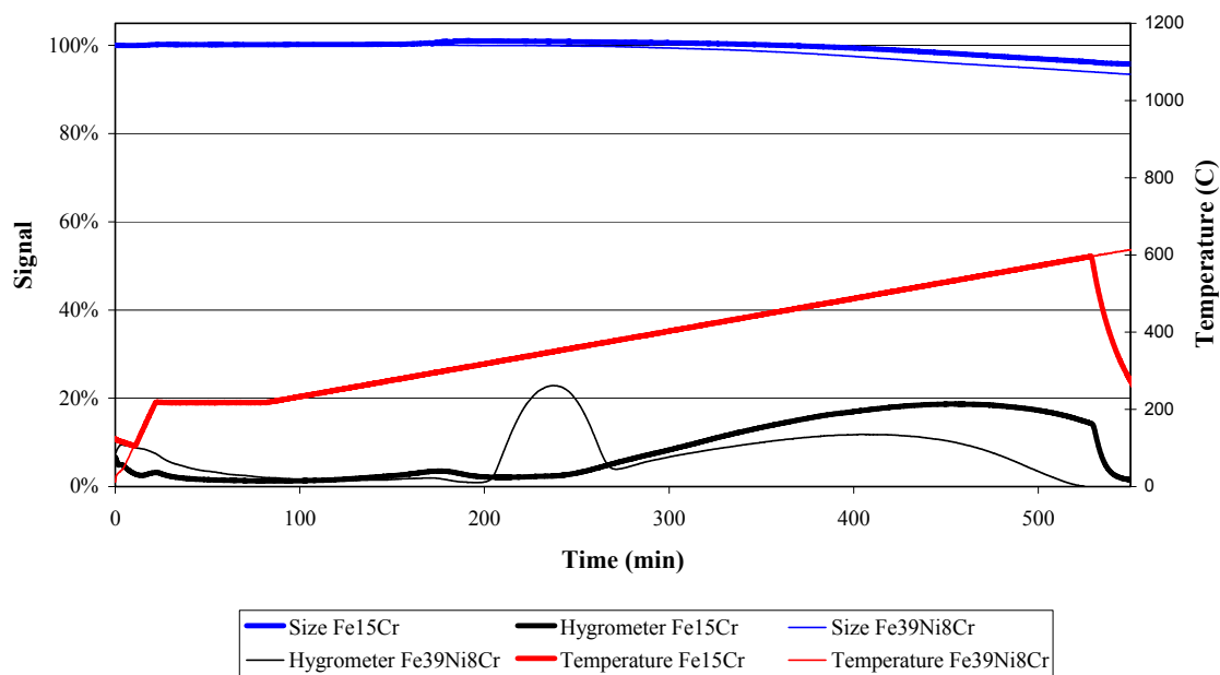
Figure 57. Sintering and reduction for Fe15Cr and Fe39Ni8Cr.
