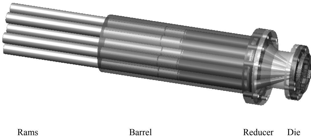
Figure C4. Multi-cavity hybrid extruder assembly.
