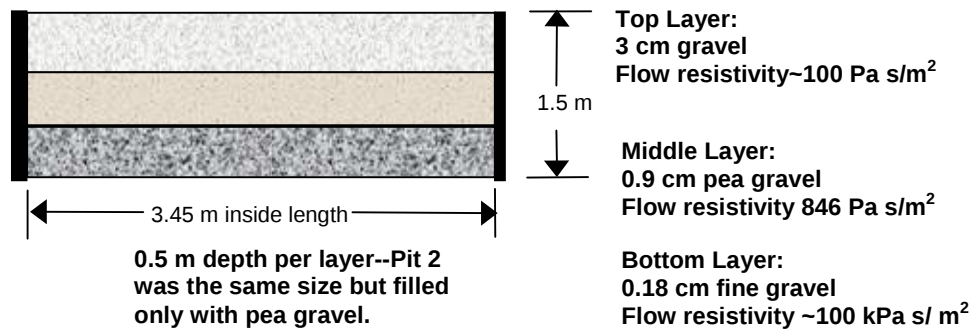
Figure 13. General dimensions and fill of Pit 1. Pit 2 was the same size but filled entirely with what was nominally 0.9-cm pea gravel.
