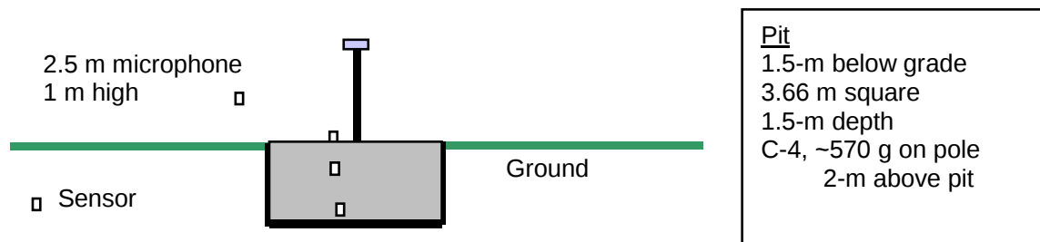
Figure 9. Elevation view of Pit 1. Pit 2 is the same except that there was no sensor at the bottom of Pit 2.
