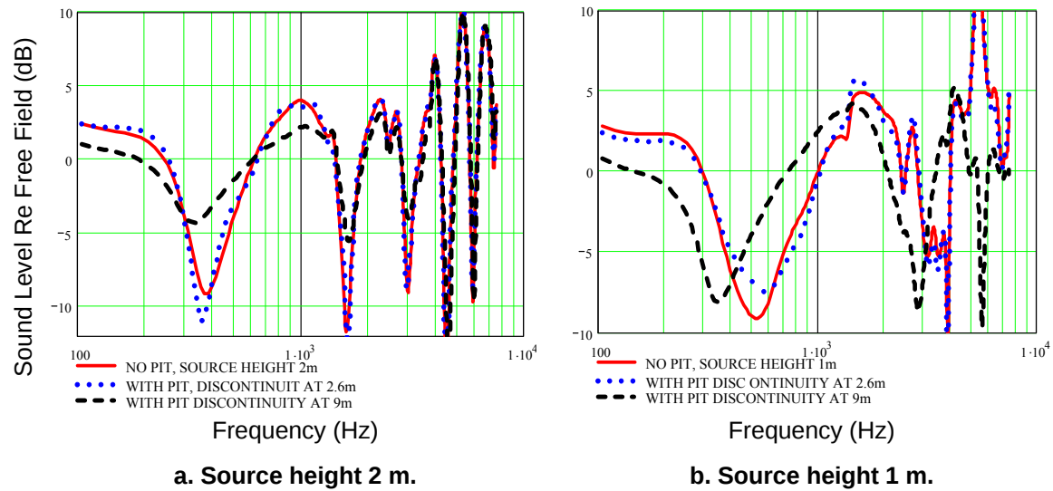
Figure 45. Predicted excess attenuation spectra: source over Pit 1.
