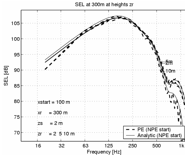
Figure 69. Linear sound exposure level at 300-m distance from the source, with the NPE start at 100 m for a maximum height of the NPE grid.
