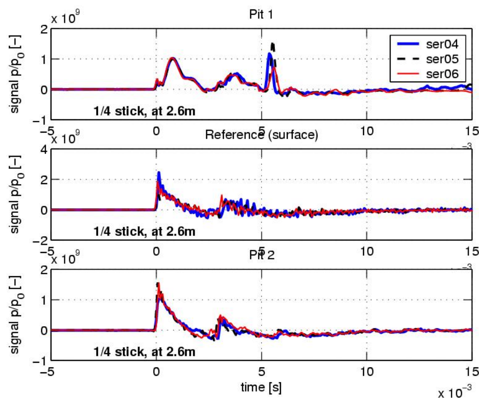
Figure 23. Comparison of three pancake recordings. Time signals have been shifted so that at t = 0 , the first pressure rise occurs. Note that for the upper plot a sharp pressure rise is nearly absent.
