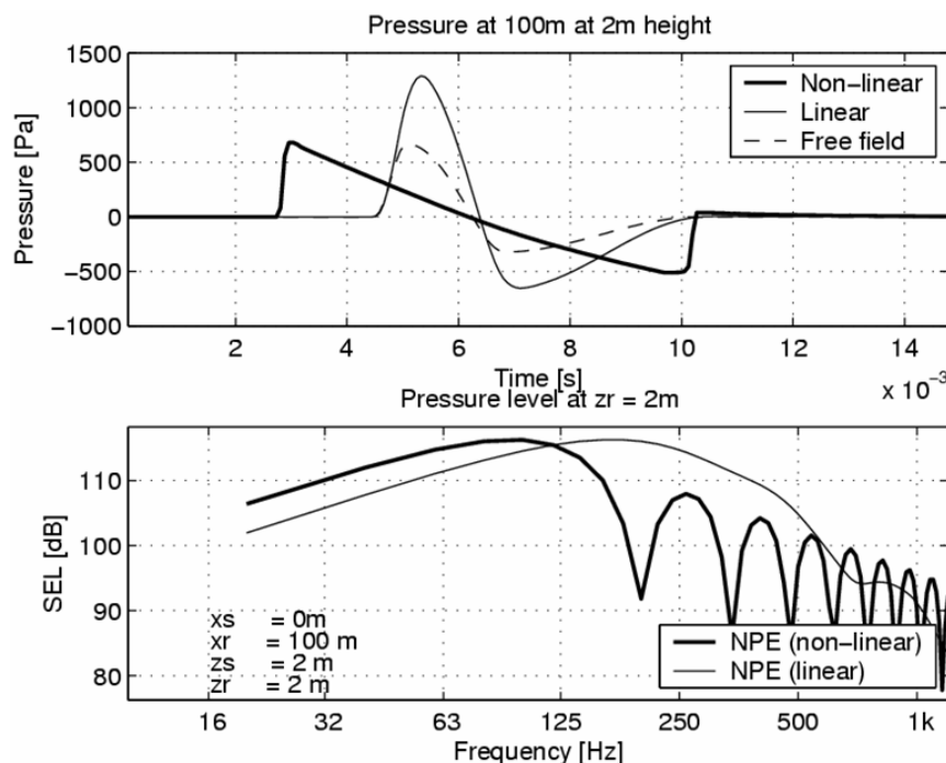
Figure 67. NPE results at 100 m for non-linear propagation above a rigid ground, linear propagation above a rigid ground, and linear free-field propagation. The upper graph shows the pressure–time history. The lower graph shows the spectrum (linear frequency spacing of 20 Hz).
