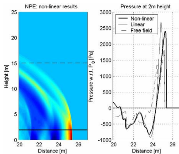
Figure 64. NPE results at 25 m from the source.
