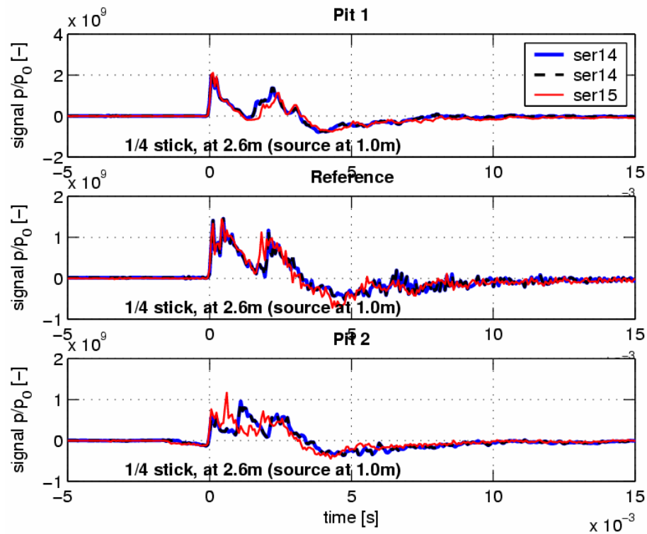
Figure B5. Pressure-time histories for the quarter-stick size at 2.6 m. The source was at 1.0-m height. Note: series 13 could not be used here.
