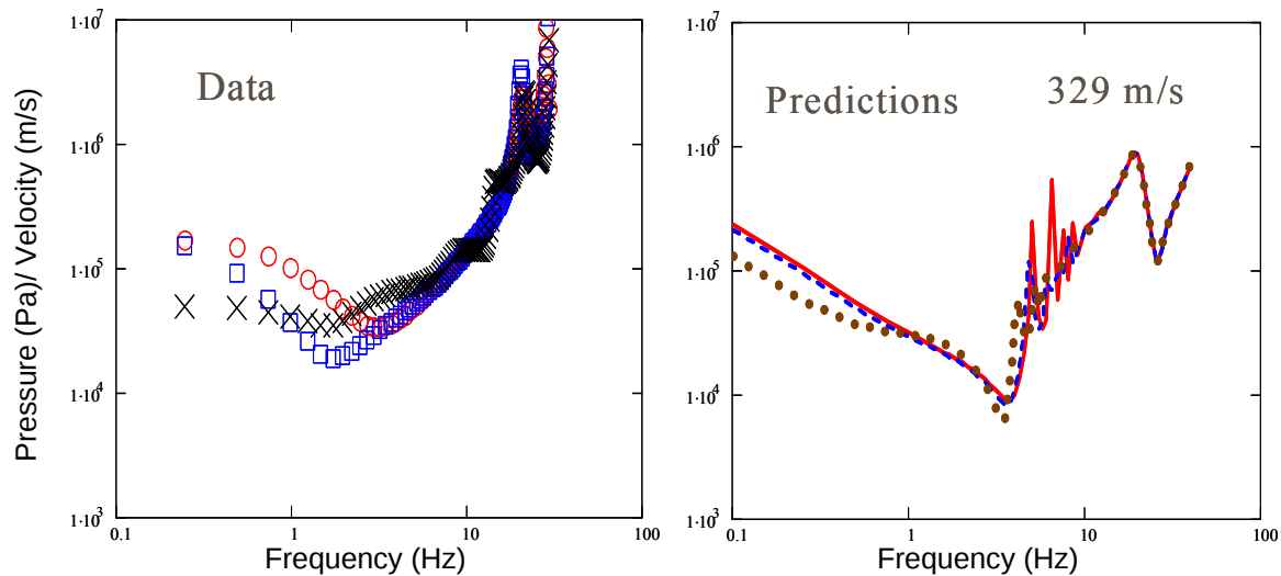
Figure 52. Acoustic-seismic coupling ratios deduced from measurements and predicted by FFLAGs at ranges of 6300 m (circles and solid line), 7200 m (boxes and broken line), and 12600 m (crosses and dotted line) assuming a sound speed in air of 329 m/s.
