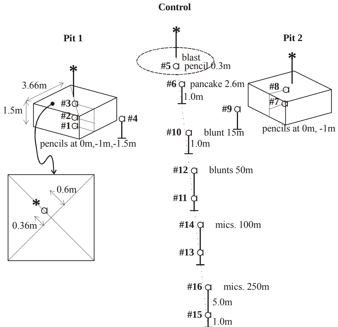
Figure 10. Overall Test I site layout. The numbers by each gauge are channel numbers for data recording and analysis.
