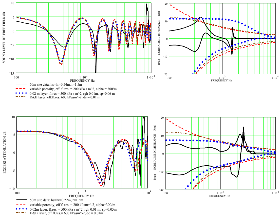
Figure 30. Two examples of the results from measurements near the 50-m mast site in the Test I area. The two graphs on the left are measured excess attenuation spectra, and the two graphs on the right are the corresponding impedance fit. (Fit parameters at the 50-m area: 2-para: \sigma_e = 200 \text{ kPa s m}^{-2} ; a = 300 /m; rough 5-para: \sigma = 500 \text{ kPa s m}^{-2} ; \Omega = 0.4 , T = 1/\Omega , r_{gh} \text{ ht} = 0.015 \text{ m} , sp = 0.05 \text{ m} , d = 0.05 \text{ m} ; Delany & Bazley \sigma_e = 600 \text{ kPa s m}^{-2} ; d_e = 0.01 \text{ m} .)
