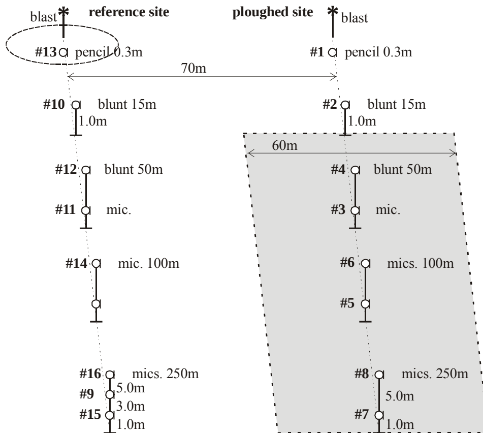
Figure 16. Overall Test II site layout. The numbers by each gauge are channel numbers for HP data analysis.
