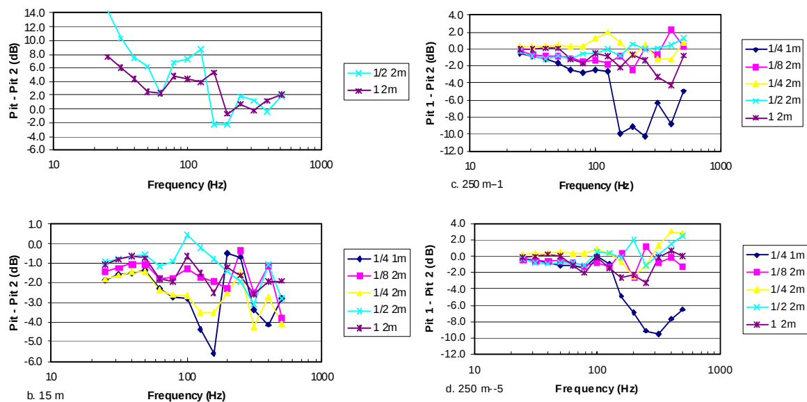
Figure 28. Plots of Pit 1 minus Pit 2 values as functions of frequency for the charge indicated. Here, the quarter-stick charge at a height of 1 m clearly departs from the other data at all three distances.
