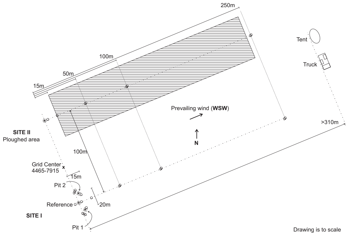
Figure 17. Overall layout for the combined Test I and Test II experiments.
