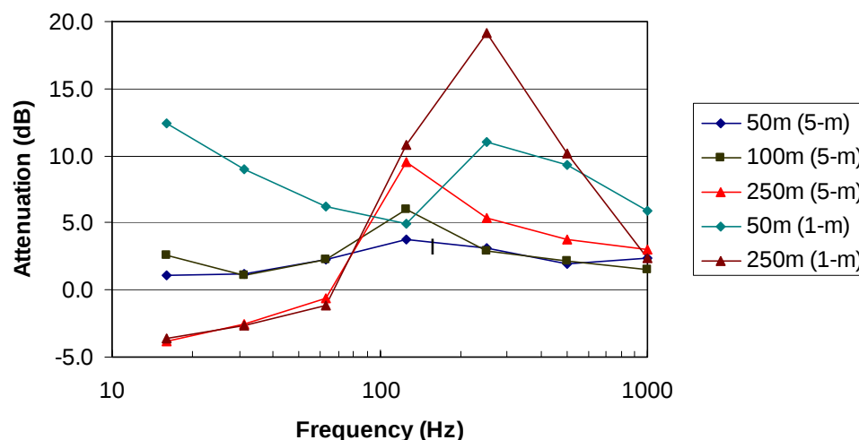
Figure 29. Plots of the average differences between the control (grass) field and the plowed field from Table 8.
