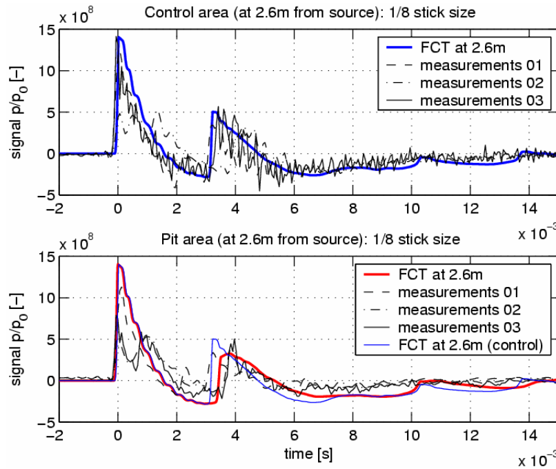
Figure 56. Comparison of numerical and measured pressure-time histories for the eighth-stick size at 2.6-m distance. The upper graph shows the control data, while the lower graph shows Pit 2 data. The first peak of the normalized pressures ( p_0 = 20 \mu\text{Pa} ) has been shifted in time and set to zero for comparison. The microphone height is 1.0 m.
