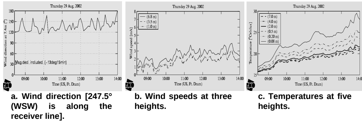
Figure 48. Variation of meteorological conditions with time during the tests.
