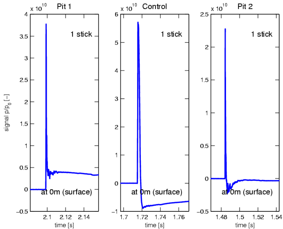
Figure 39. Waveforms recorded at the surface for the one-stick charge.
