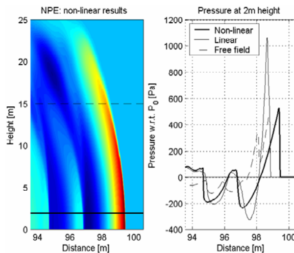
Figure 65. NPE results at 100 m from the source.
