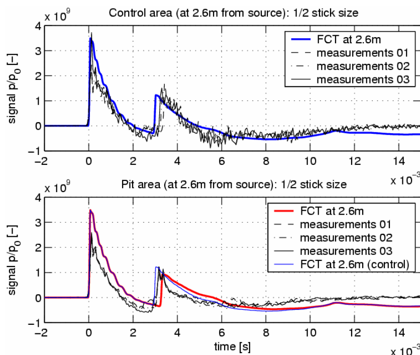
Figure 57. Comparison of numerical and measured pressure-time histories for the half-stick size at 2.6-m distance. The upper graph shows the control data, while the lower shows the Pit 2 data. The first peak of the normalized pressures ( p_0 = 20 \mu\text{Pa} ) has been shifted in time and set to zero for comparison. The microphone height is 1.0 m.
