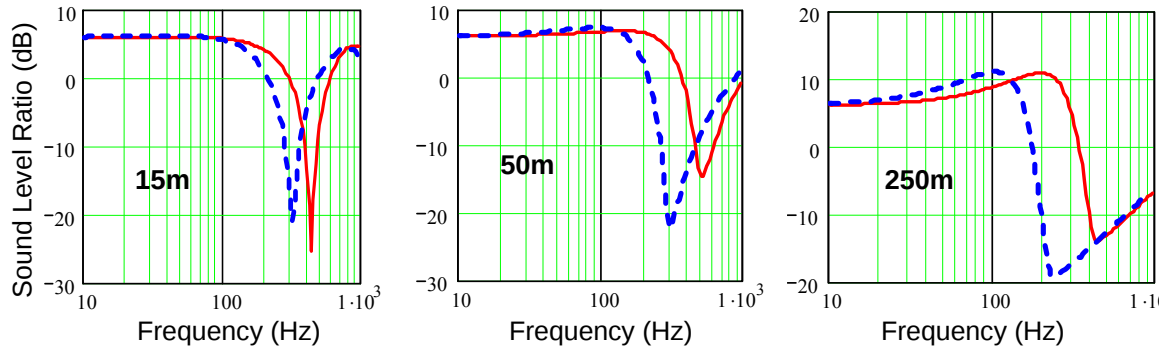
Figure 47. Predicted excess attenuation (sound level re free field) spectra at 15, 50, and 250 m using a linear propagation model.
