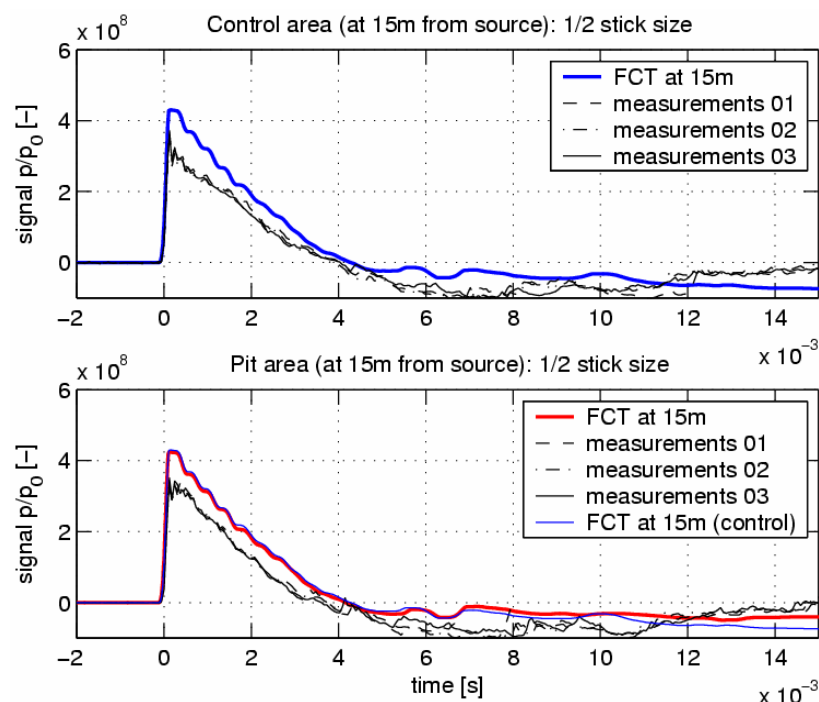
Figure 59. Comparison of numerical and measured pressure-time histories for the half-stick size at 15-m distance. The upper graph shows the control data, while the lower graph shows the Pit 2 data. The first peak of the normalized pressures ( p_0 = 20 \mu\text{Pa} ) has been shifted in time and set to zero for comparison. The microphone height is 1.0 m.
