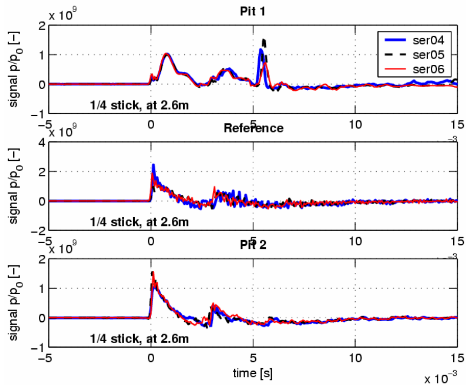
Figure B2. Pressure-time histories for the quarter-stick size at 2.6 m. The source was at 2.0-m height.
