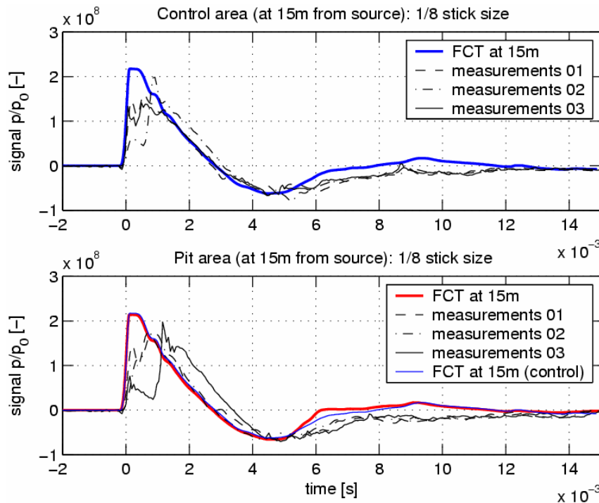
Figure 58. Comparison of numerical and measured pressure–time histories for the eighth-stick size at 15-m distance. The upper graph shows the control data, while the lower graph shows the Pit 2 data. The first peak of the normalized pressures ( p_0 = 20 \mu\text{Pa} ) has been shifted in time and set to zero for comparison. The microphone height is 1.0 m.
