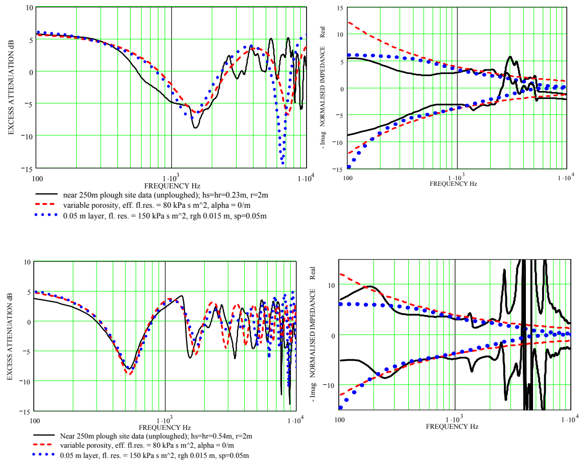
Figure 31. Two examples of measurements near the 250-m mast site in the Test II area (before plowing) and various model predictions. The two graphs on the left are measured and predicted excess attenuation spectra, and the two graphs on the right are corresponding impedance fits.
