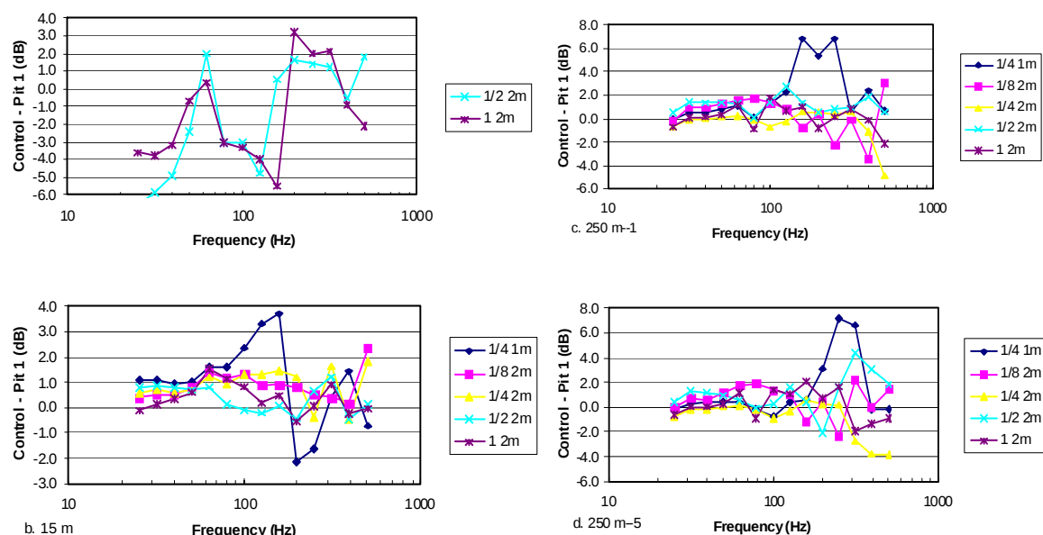
Figure 26. Plots of Control minus Pit 1 values as functions of frequency for the charge indicated. Note that the quarter-stick charge at a height of 1 m clearly departs from the other data at both 15 and 250 m.
