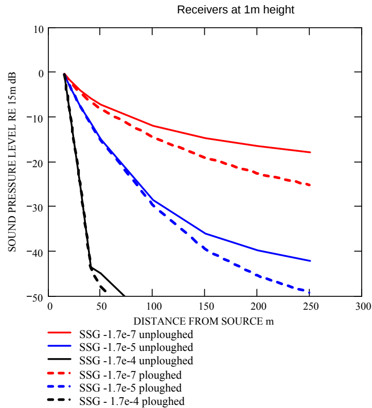
Figure 50. Residue series predictions of the sound levels relative to 15 m at 1-m-high receivers for three different effective sound speed profiles and for a broad-band source.
