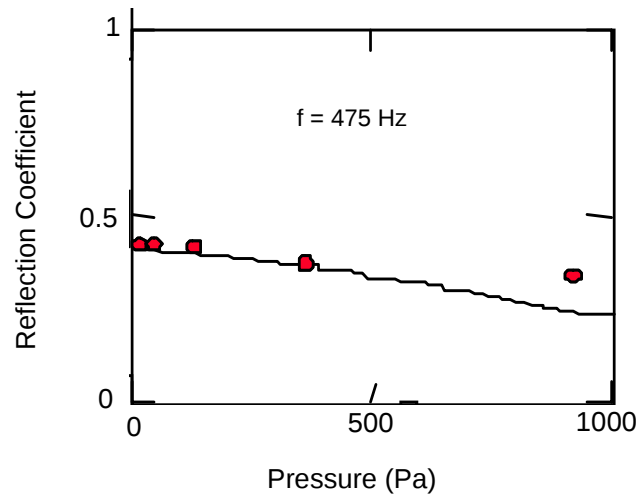
Figure 4. Decrease in reflection coefficient for increasing pressure for 15-cm-thick hard-backed 9-mm gravel at 475 Hz. The line show predicted values; the points show measured values. (From Umnova et al. 2003.)
