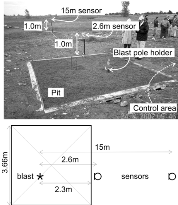
Figure 53. Measurement set-up for C4 explosives above Pit 2.
