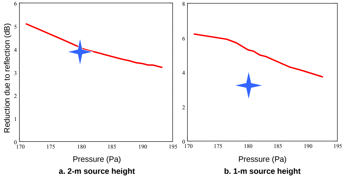
Figure 42. Predictions (red lines) for reduction in amplitude due to reflection from Pit 2 compared to data (blue stars) for a quarter stick.
