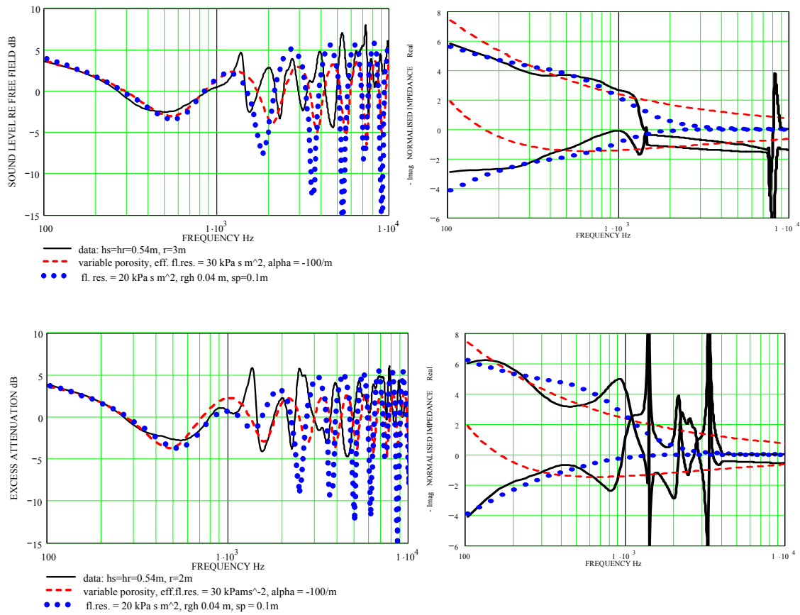
Figure 32. Excess attenuation and directly fitted impedance spectra obtained across (i.e. at right angles to) furrows of plowed sandy soil during Test II. The two graphs on the left are measured and predicted excess attenuation spectra, and the two graphs on the right are corresponding impedance fits.
