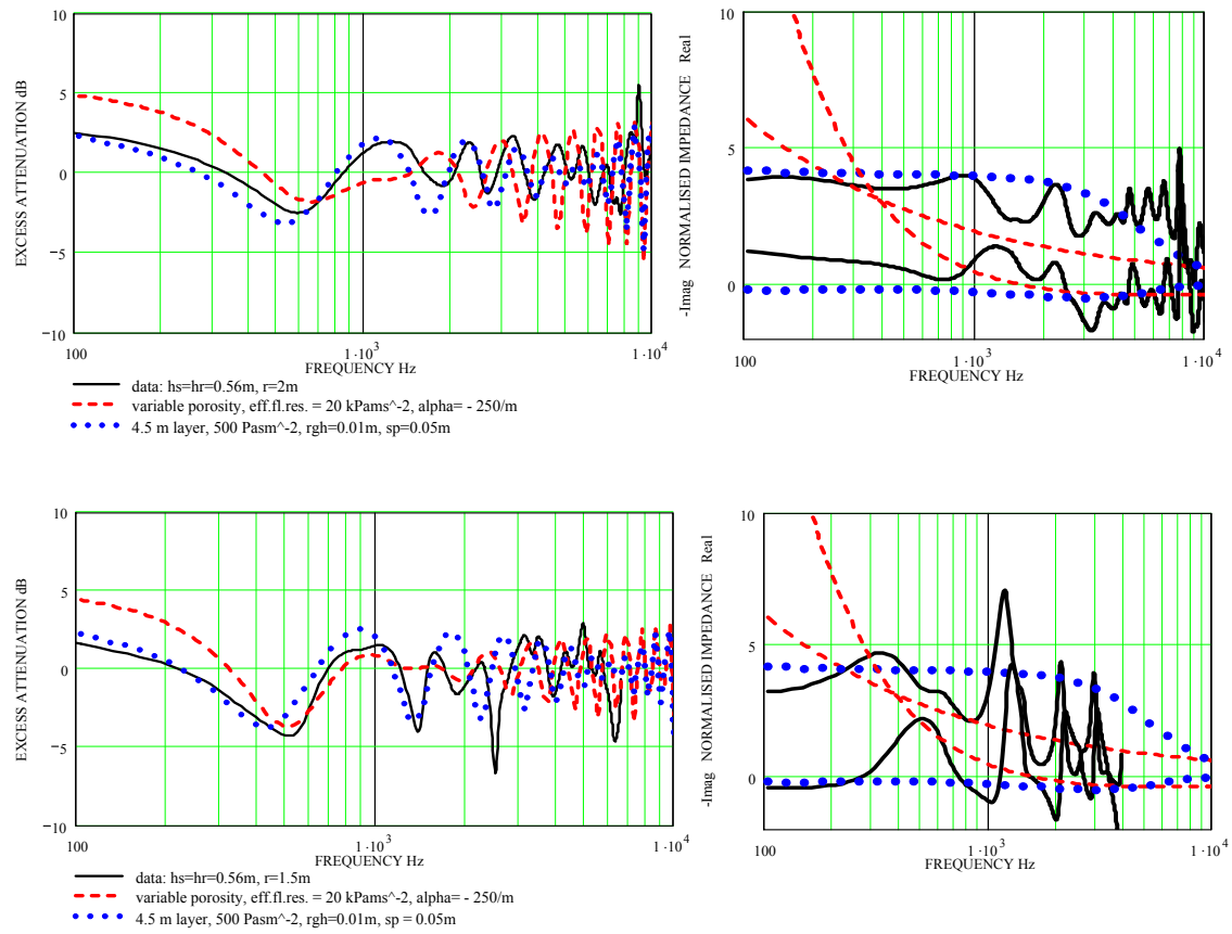
Figure 33. Excess attenuation and directly fitted impedance spectra obtained at Gravel Pit 1.
