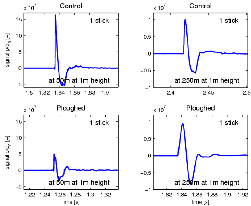
Figure 51. Pressure–time signals at 1.0 m high. The upper two graphs are for the reference site; the lower two are for the ploughed site, all for one stick.
