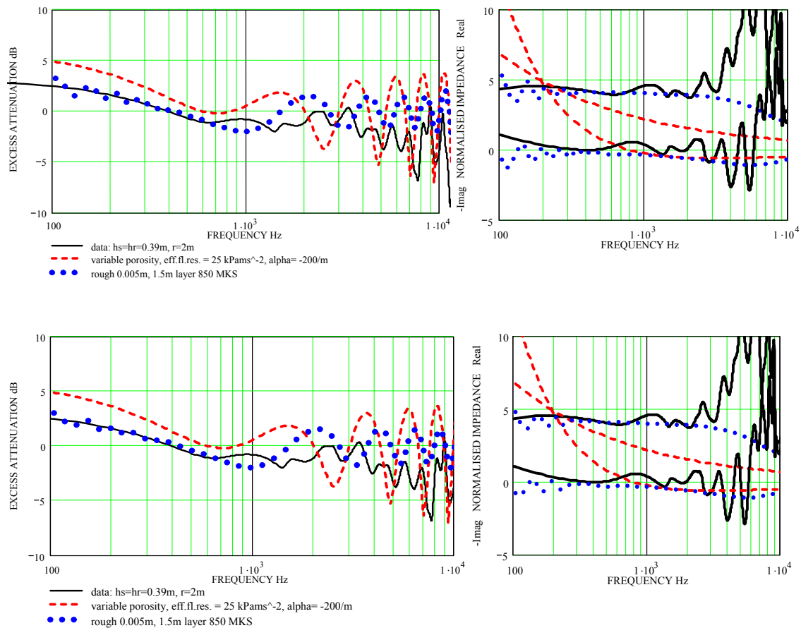
Figure 34. Excess attenuation and directly fitted impedance spectra obtained at Gravel Pit 2 using measured flow resistivity ( 850 \text{ Pa s m}^{-2} ). The top two graphs assume a hard-backed layer, and the bottom two graphs assume a non-hard-backed layer.
