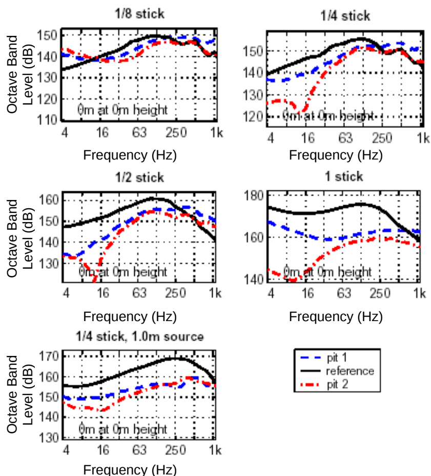
Figure 40. Octave band spectra measured at the reference site surface and at the surfaces of Pits 1 and 2 for various charge sizes (all at a source height of 2 m, except the bottom graph, which has a source height of 1 m).
