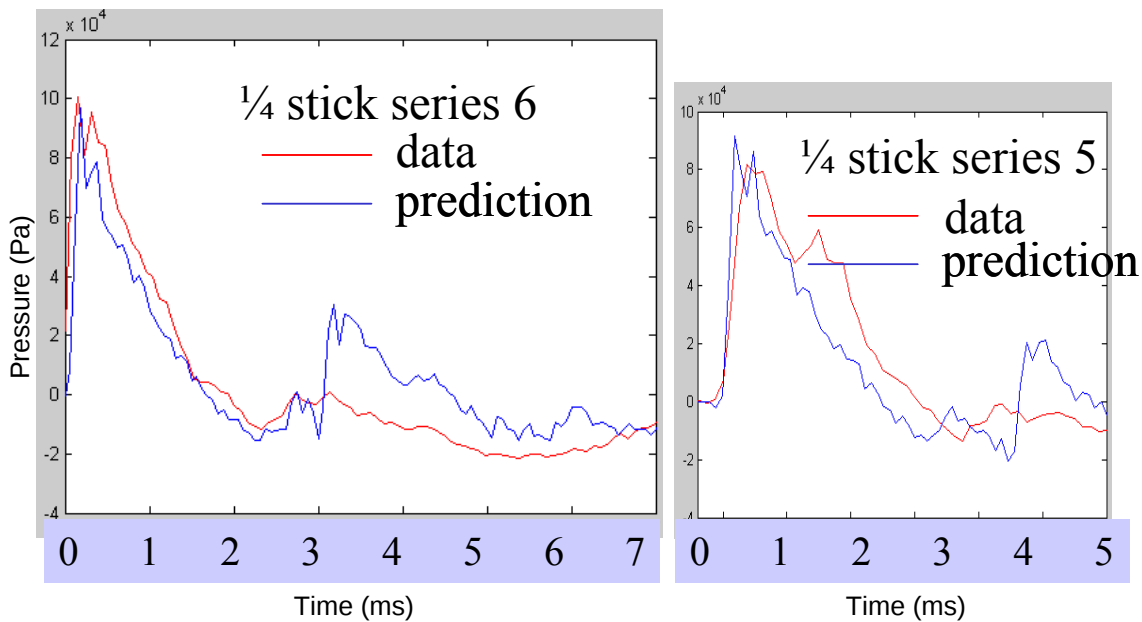
a. Quarter stick, series 6 prediction data.
