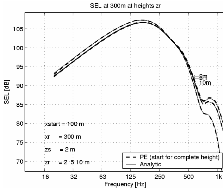
Figure 70. Linear sound exposure level at 300-m distance from the source, with the start at 100 m with maximum height as used for PE grid.
