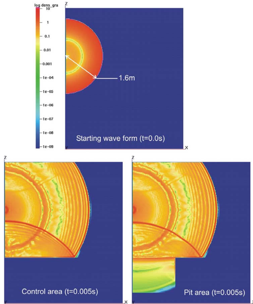
Figure 55. Density gradient calculated with the FCT code. The top image shows the starting condition, with a source at a height of 2.0 m at time t = 0.0 s. The bottom left image shows the shock wave above a rigid surface. The bottom right image shows the shock wave above absorbing Pit 2.
