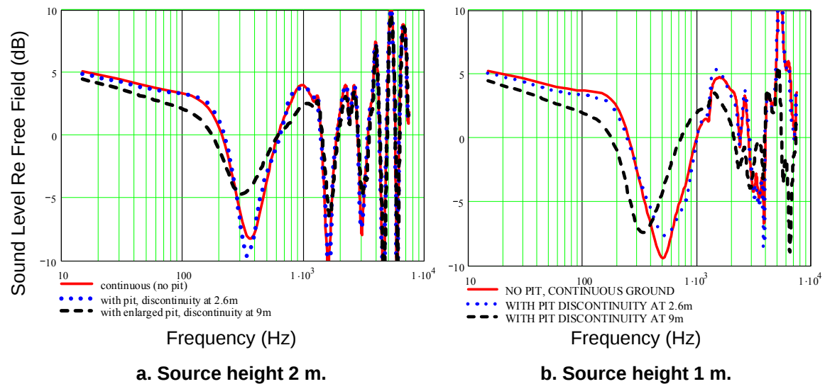
Figure 46. Predicted excess attenuation spectra: source over Pit 2.
