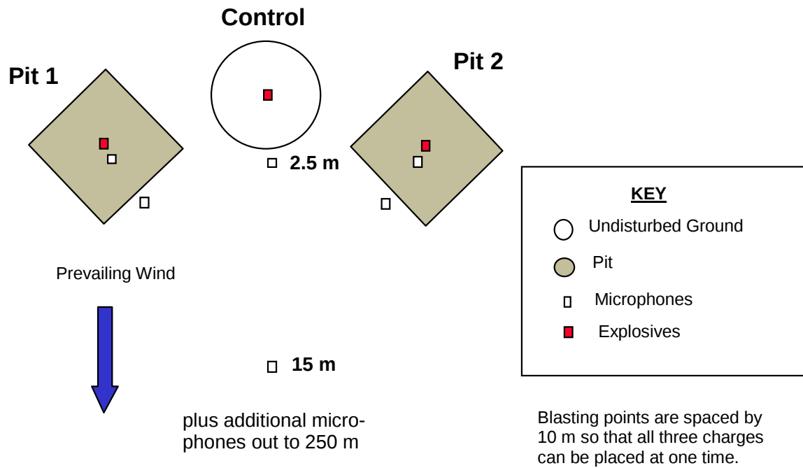
Figure 8. Plan view of the blast site area for Test I.
