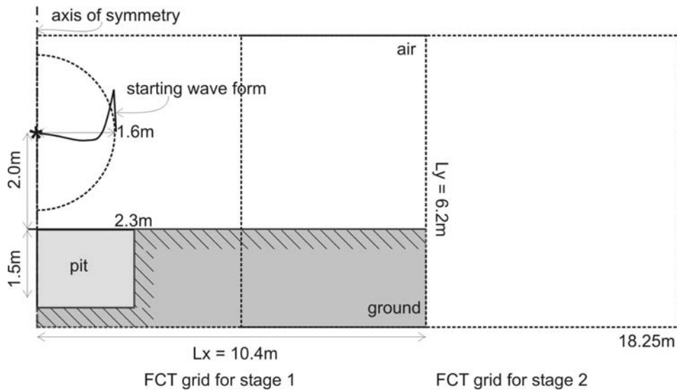
Figure 54. Numerical set-up for the FCT method. Stage 2: 4.99 to 18.25 m.
