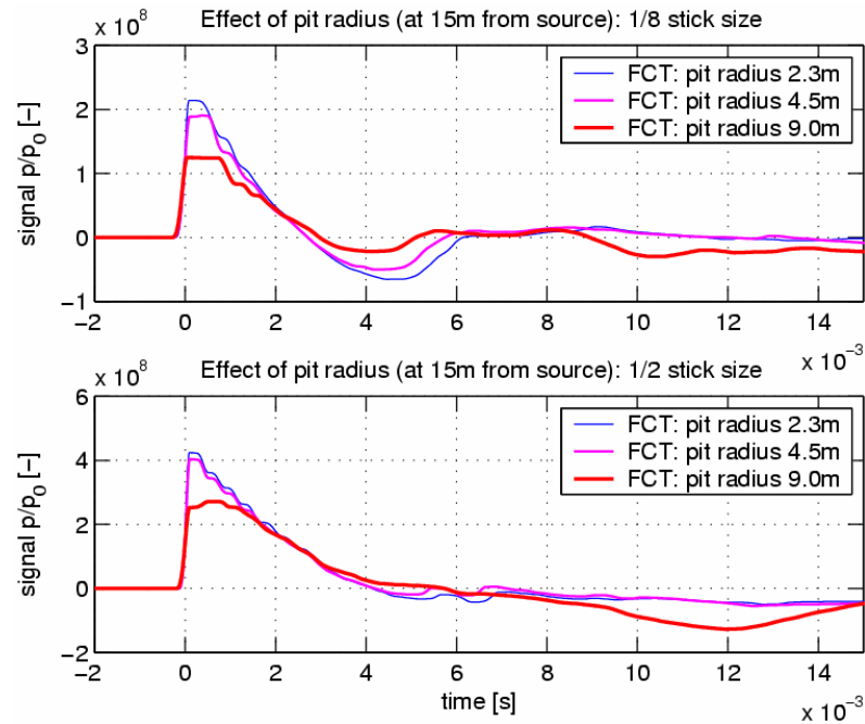
Figure 60. Calculated pressure–time histories for three pit sizes. Upper: eighth-stick size. Lower: half-stick size. Normalized pressure ( p_0 = 20 \mu\text{Pa} ) at 15 m from the source. The source was at a height of 2 m. The receiver was at a height of 1 m.
