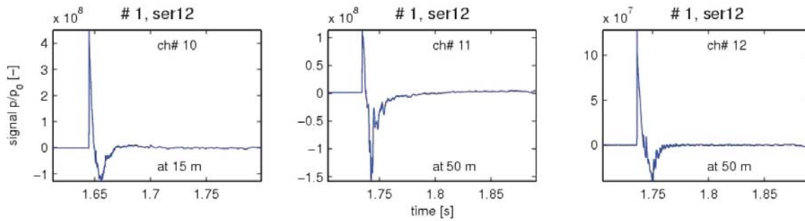
Figure 24. Pressure-time recordings for a blunt gauge for series 12 (one stick).
