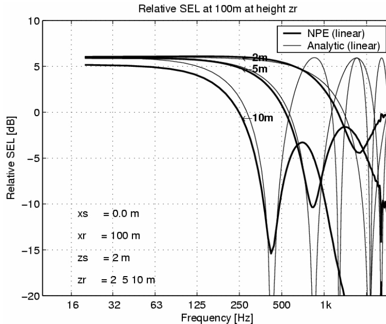
Figure 68. Comparison of the linear excess attenuation for NPE and an analytical two-ray model. The source was at 0 m at a height of 2 m. The receiver at 100 m at heights of 2, 5, and 10 m.
