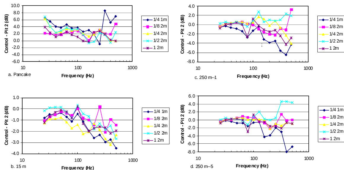
Figure 27. Plots of Control minus Pit 2 values as functions of frequency for the charge indicated. Again, the quarter-stick charge at a height of 1 m clearly departs from the other data, this time at both 2.5 and 250 m.
