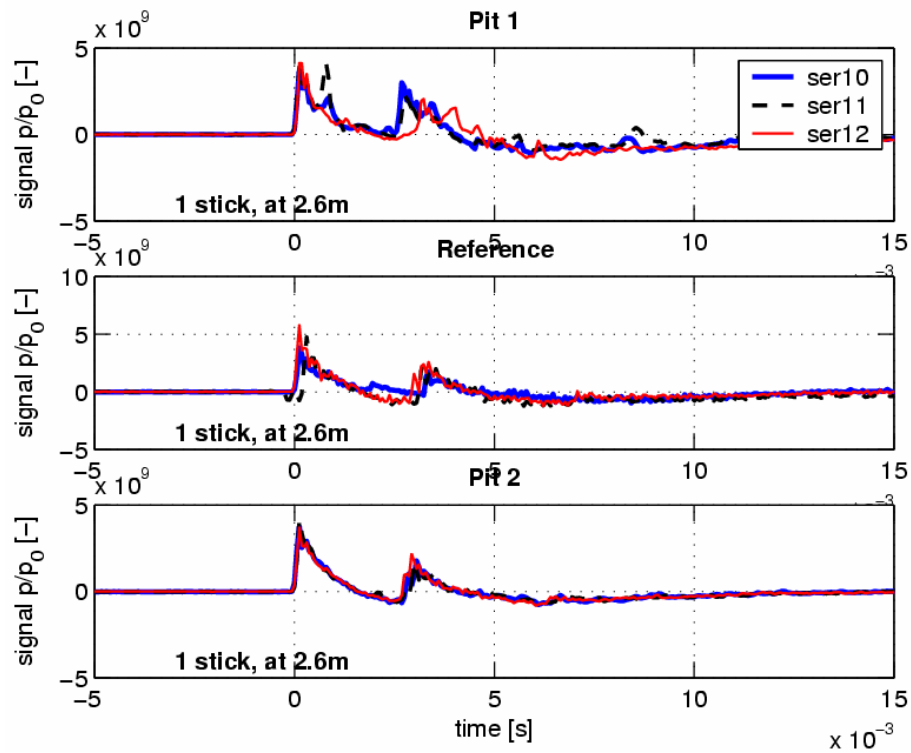
Figure B4. Pressure-time histories for the one-stick size at 2.6 m. The source was at 2.0-m height.
