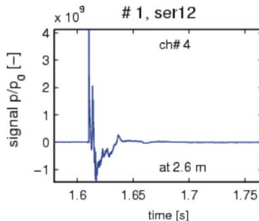
Figure 22. Typical pressure–time history for a pancake gauge (one stick—series 12).
