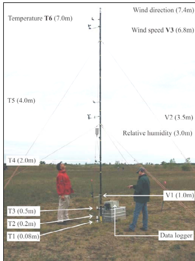
Figure 18. Meteorological sensing.
