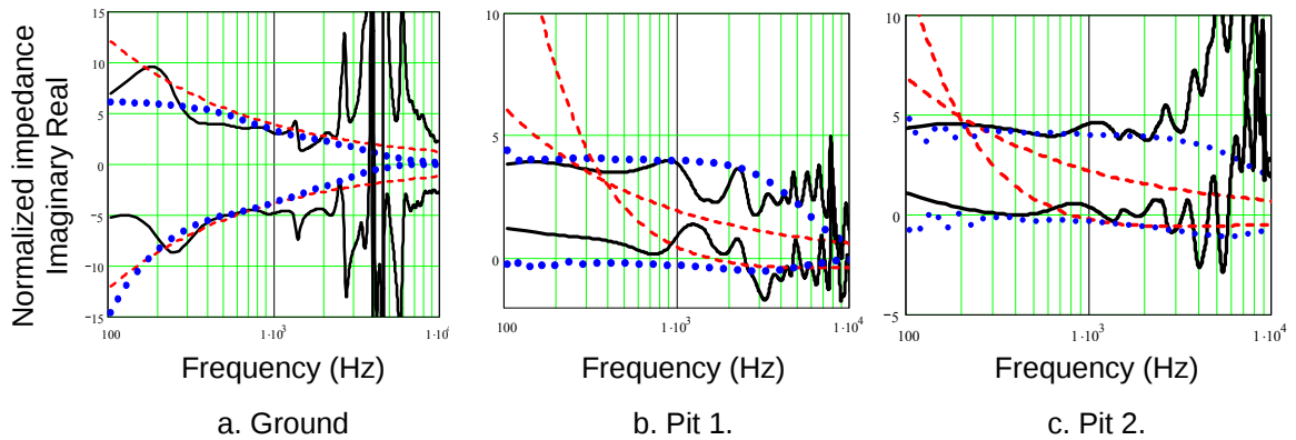
Figure 44. Impedance spectra used to describe pits and ground.
