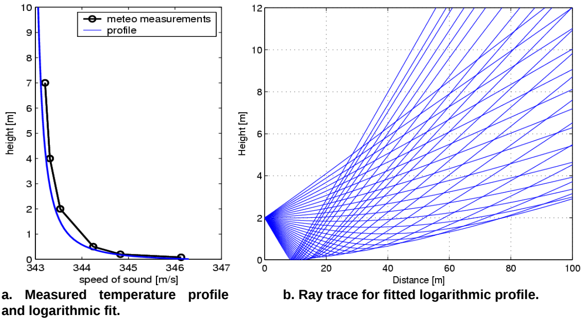
Figure 49. Speed of sound as a function of height, and effect of the temperature gradient on sound rays.
