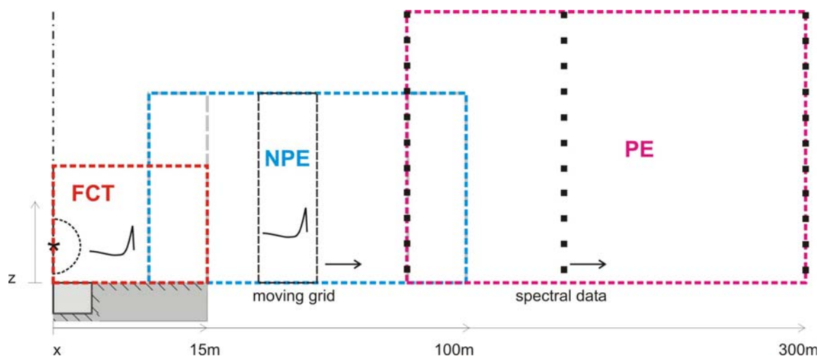
Figure 61. Schematic overview of coupling of FCT with NPE and PE.
