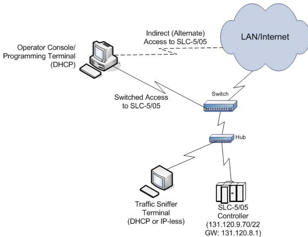
Figure 18 Network Topology
