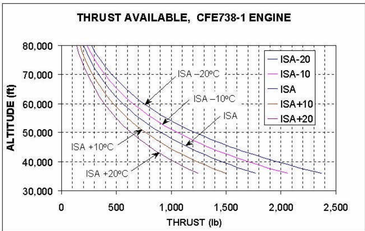
Figure 7. Engine Thrust v. Altitude
