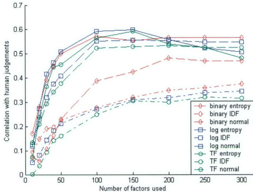
Figure 6: Correlation between stopped, backgrounded LSA and human judgements.
