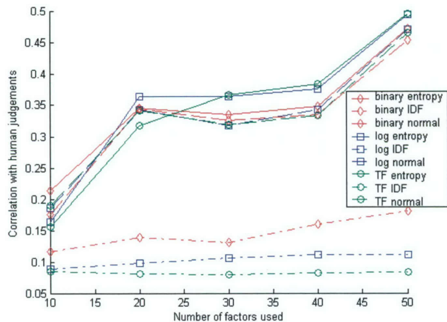
Figure 3: Correlation between unstopped LSA and human judgements.
