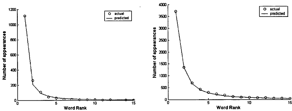
Figure 1: Expected and actual frequency spectrum for 50 and 364 ABC newsmail documents.
