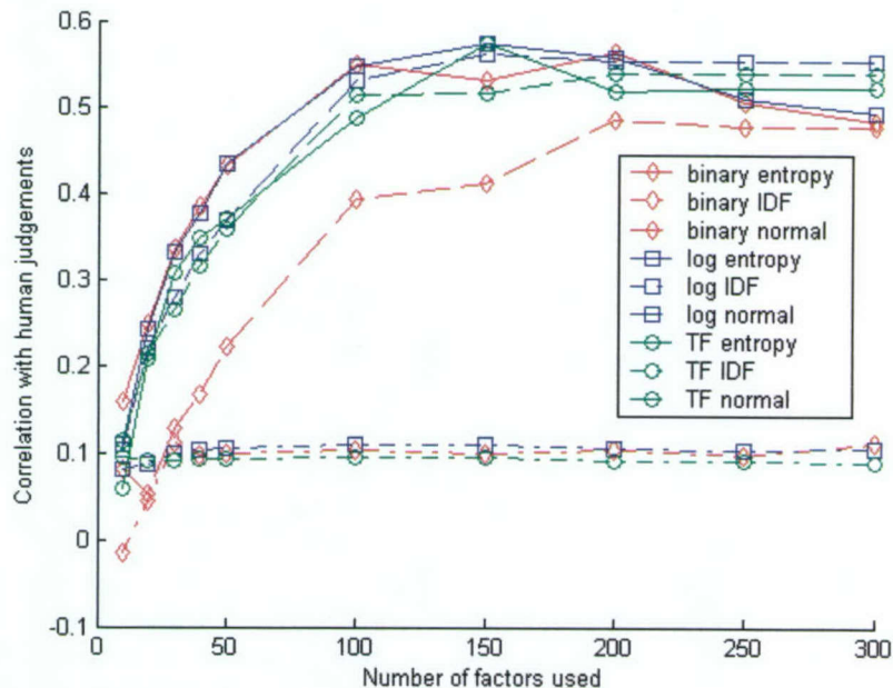
Figure 5: Correlation between unstopped, backgrounded LSA and human judgements.
