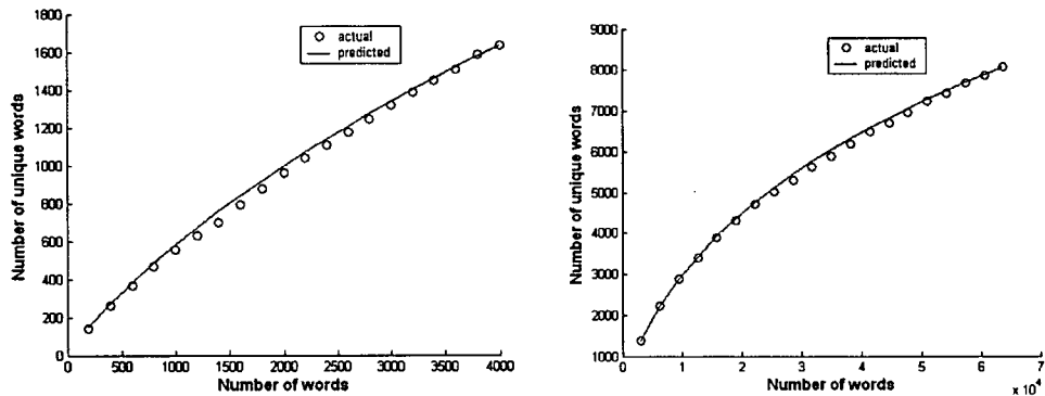
Figure 2: Expected and actual vocabulary growth in the 50 and 364 ABC newsmail documents.
