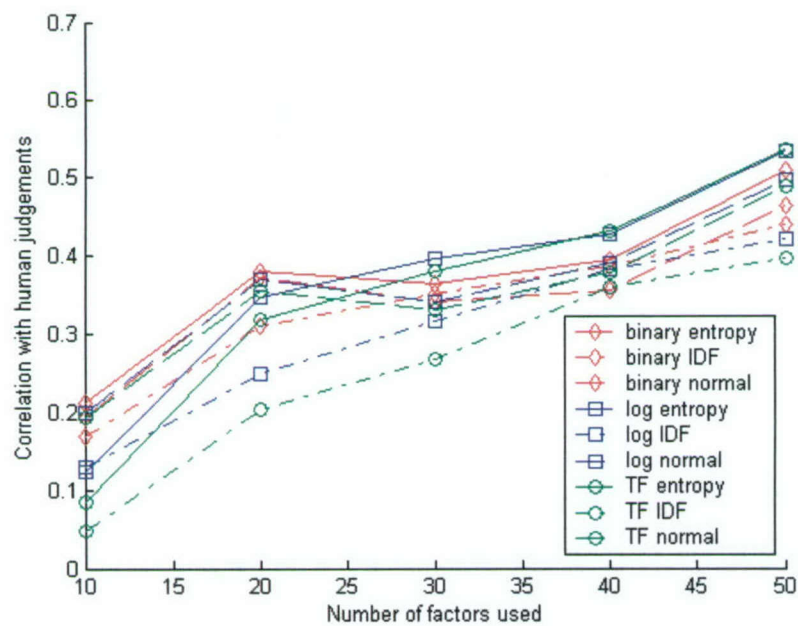
Figure 4: Correlation between stopped LSA and human judgements.
