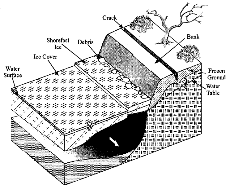
Figure 21. Combined hydraulic impacts (e.g., thalweg shift and bank-toe erosion) and geomechanical impacts (e.g., freeze-thaw weakening of bank material, elevated seepage pressures, bankfast-ice loading) may weaken and erode channel banks, especially along channel bends, and result in continual, overall channel destabilization.
