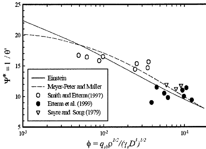
Figure 12. Bedload data compared with curves generated using Einstein's procedure and Meyer-Peter and Müller formula developed from open water data. Covered flow data conform to the same curves developed using open water data.
