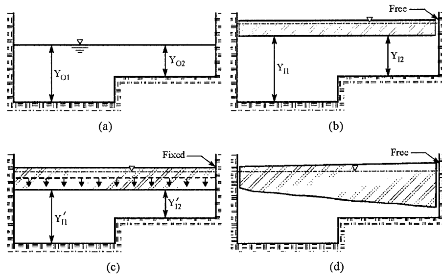
Figure 3. An ice cover may reduce open water proportions (a) of flow conveyance in lateral segments of a two-part compound channel if the cover is level and free floating (b); increase them if the cover is fixed and thickens (c); or, increase them if the cover is not uniformly thick (d).
