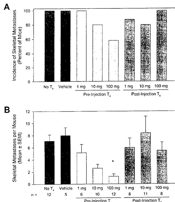
Figure 5. Overall number of 435 GFP skeletal metastases are significantly ( P = 0.002 ) reduced in a dose-dependent manner following pre-treatment of mice with S247. Mice were treated as depicted in Figure 1. (A) Percent of mice having at least one skeletal metastasis (includes: skull, mandible, ribs, vertebrae, scapula, humerus, radius, ulna, pelvis, femur and tibia.). (B) The number (mean \pm SEM) of skeletal metastases per mouse. *Significantly different from vehicle.
