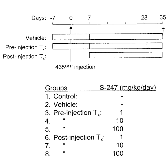
Figure 3. Schematic representation for in vivo analysis of S247 effects on breast cancer metastasis to bone. S247 treatment (Tx) using mini-osmotic pumps began one week prior to, or one week after, inoculation of 435 GFP cells ( 2 \times 10^5 ). Mice were euthanized and necropsied five weeks following tumor cell injection and examined for fluorescent skeletal metastases ( \dagger ).
