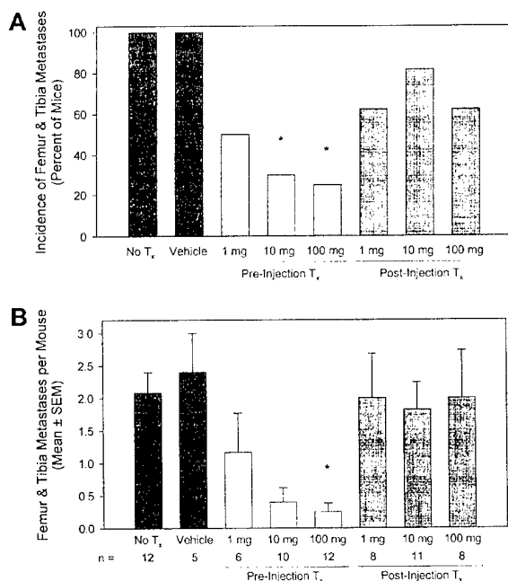
Figure 4. Incidence and number of 435 GFP femur and tibia metastases are significantly ( P = 0.002 ) reduced in S247 pre-treated mice. Female athymic mice were treated with S247 (1, 10 or 100 mg/kg/day) starting either one week prior to (pre-injection T x ) or one week subsequent to (post-injection T x ) intracardiac injection of 2 \times 10^5 435 GFP cells. Mice were euthanized and necropsied five weeks after tumor cell injection. Fluorescent metastases in intact bones were recorded. (A) Percent of mice exhibiting at least one metastasis in a femur or tibia. (B) The number (mean \pm SEM) of metastases to femur and tibia per mouse. *Significantly different from vehicle.
