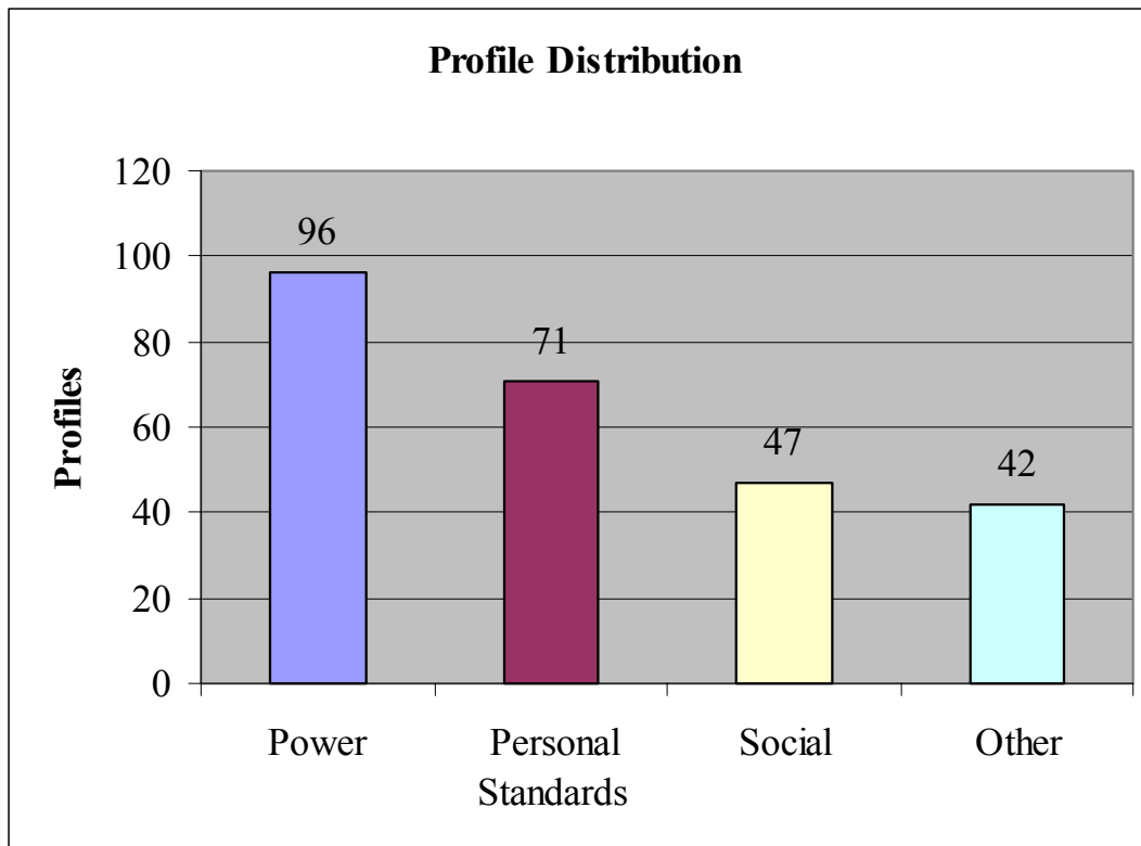
Figure 10. Profile Distribution
