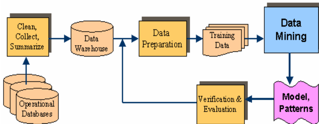
Figure 2. The Data Mining Process (From: http://www-users.cs.umn.edu/~mjoshi/hpdmmtut/sld001.htm . October 2003)
