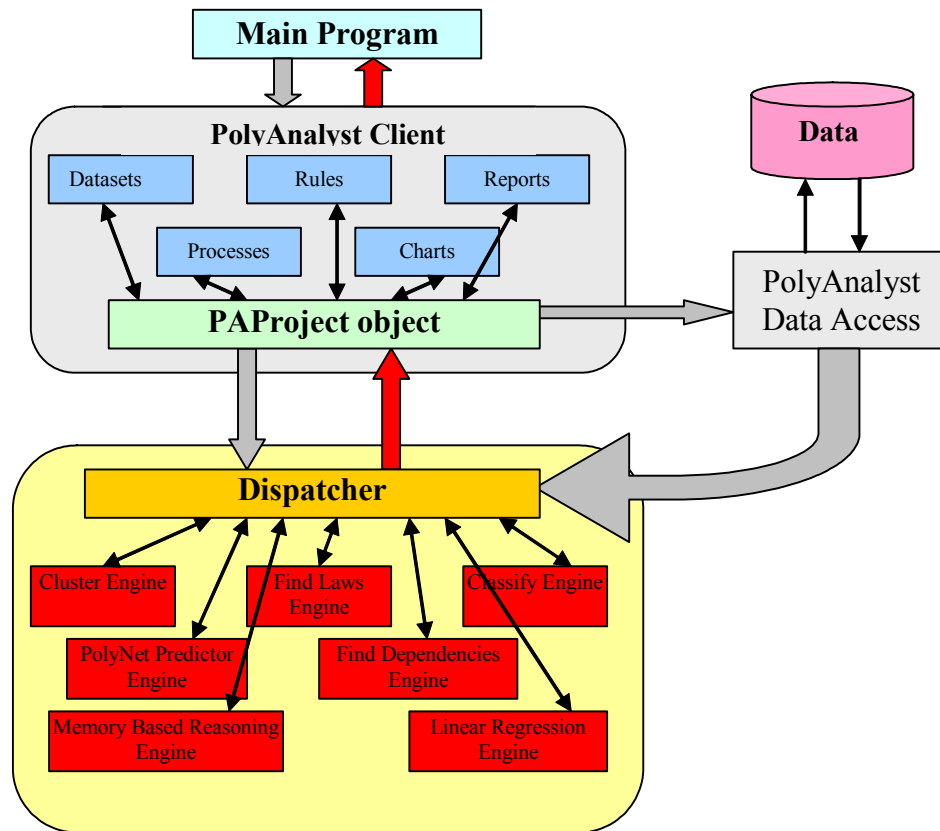
Figure 7. PolyAnalyst 4.6 Machine Learning Algorithms (From: Megaputer. PolyAnalyst 4 User Manual. August 2003.)
