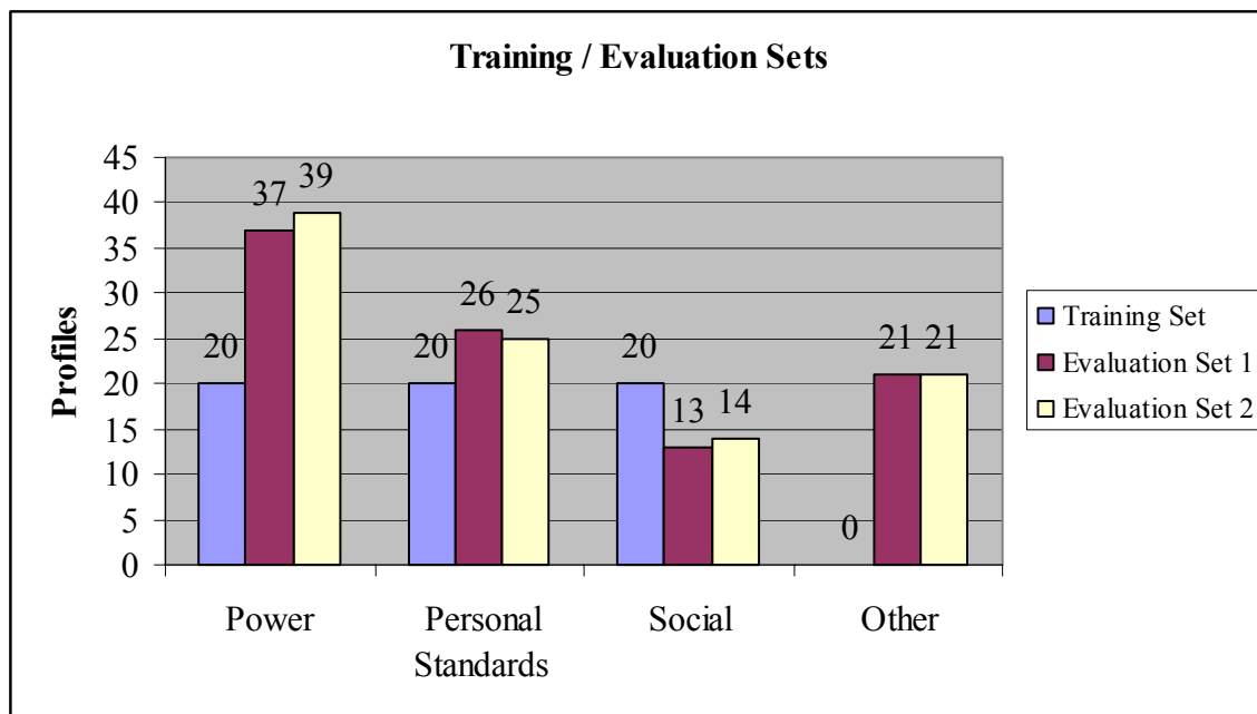
Figure 11. Training/Evaluation Sets
