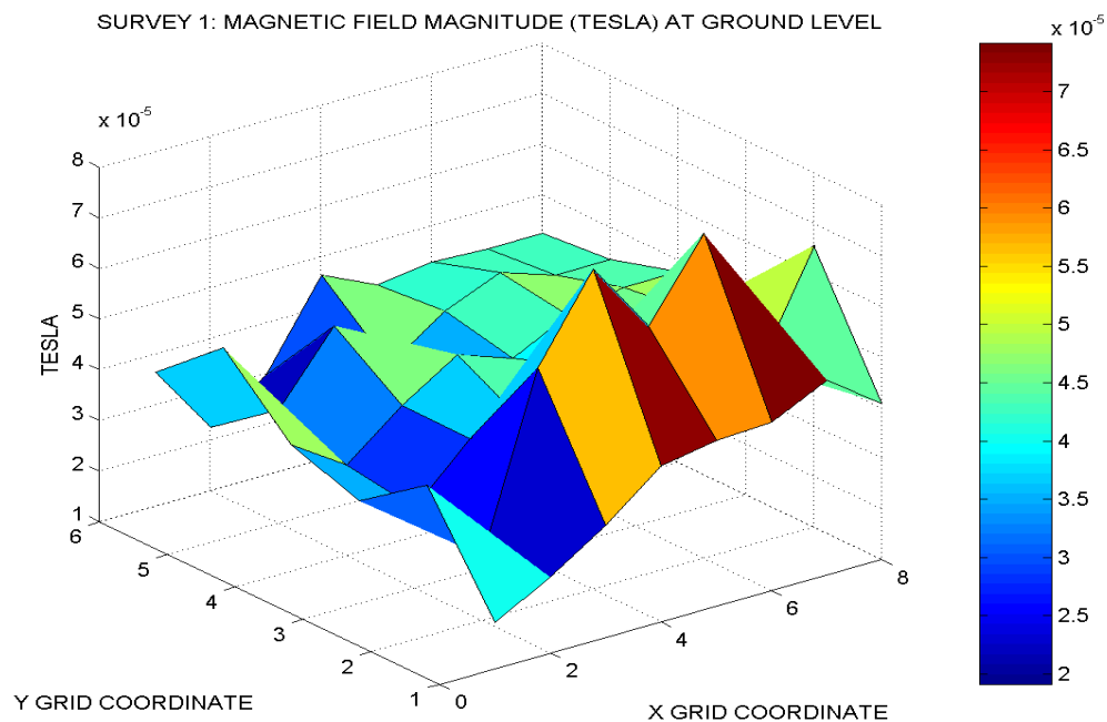
Figure 4.6 NPSAT1 Air-Bearing Laboratory Magnetic Field Survey 1 Contour Plot at Floor Level
