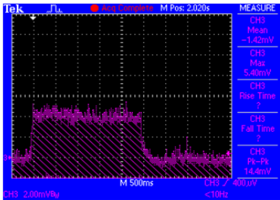
Figure 5.11 NPSAT1 Torque Driver Circuit Board Current Test (Bit level 1)
