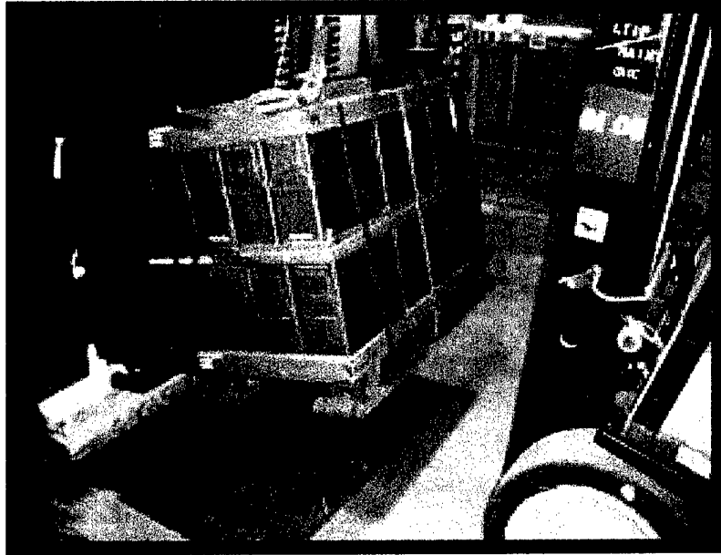
Photo 8. Test Setup for Edgewise Rotational Drop Testing.
