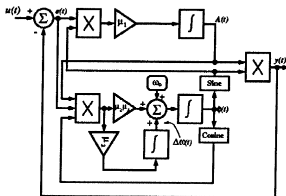
Figure 7.9. Block diagram implementation of the fundamental extraction algorithm [7.16].
