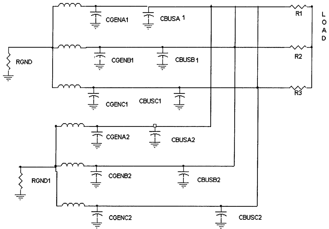
Figure 2.4 Schematic of the Configuration 2
