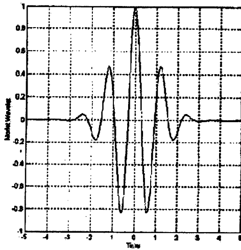
Fig 8.7. Mother Wavelet
