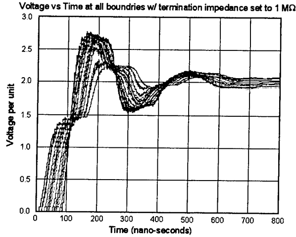
Figure 6.26. Voltage vs. Time diagram for all 18 boundaries.
