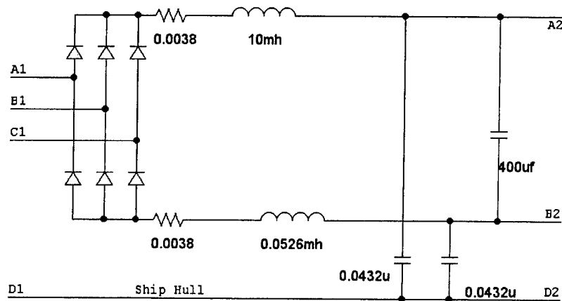
Figure 7.3. The rectifier, line impedance and filter
