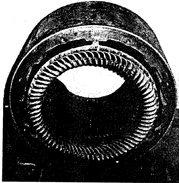
Figure 6.3. 150 HP, 3-phase, form wound induction motor used as test motor.
