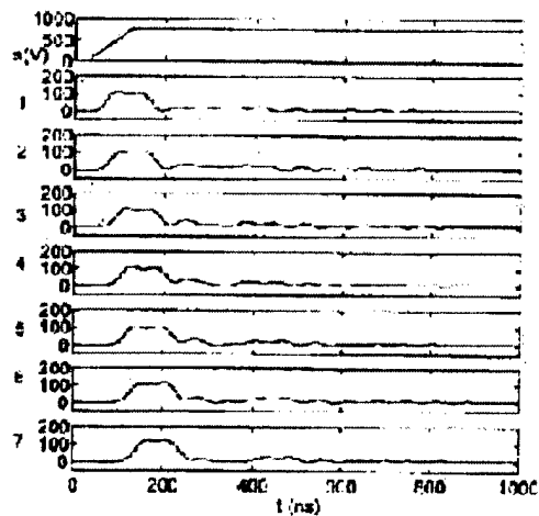
Fig 8.6. Turn-to-Turn Voltage Distribution (100ns Rise Time)
