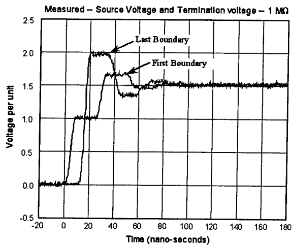
Figure 6.23. Measured results at points 'A' and 'B'.
