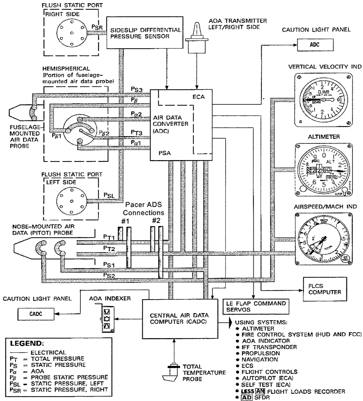
Figure 1. F-16B Production ADS with Pacer Connections
