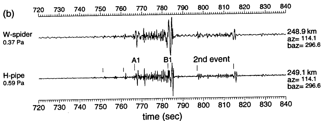
Figure 11. (a) Same as Figure 10 for Ekibastuz mine blast on Nov. 27, 1997. This event is actually two closely spaced explosions which produce overlapping Lg phases in the seismic channels but produces separate infrasound arrivals. An additional infrasound arrival at t \sim 460 s is from an earlier Ekibastuz event. (b) Blow up of the infrasound signals shown in (a). Each event is seen to consist of a sequence of pulses of increasing amplitude lasting 20-30 s.
