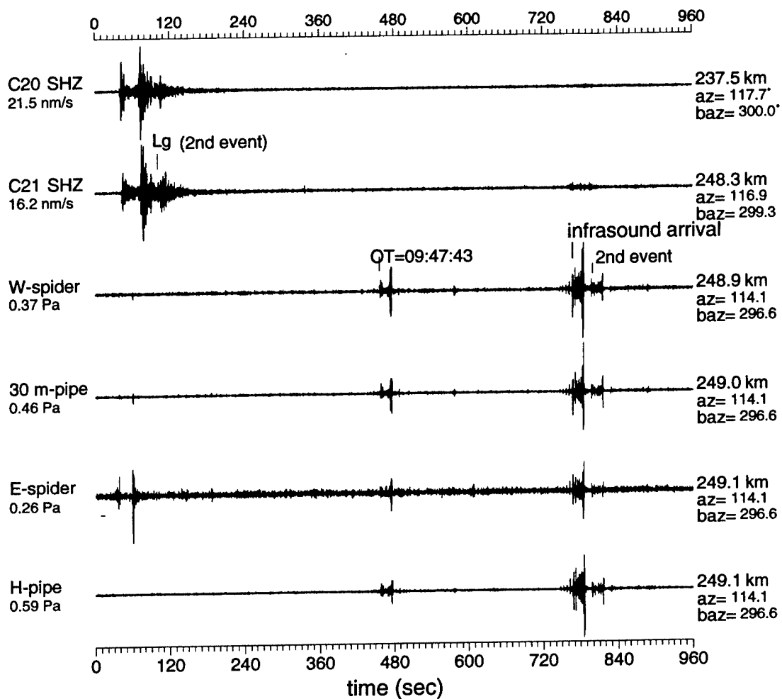
(a) 1997 Nov 27, 09:53:16 (GMT), 51.67°N, 75.40°E, Ekibastuz mine blasts
