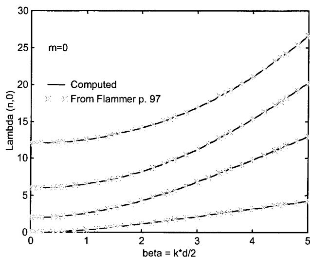
Figure 2. Eigenvalue computation.
