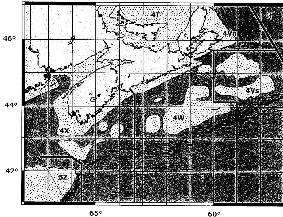
Fig. 1 — NAFO fishing areas surrounding Nova Scotia
