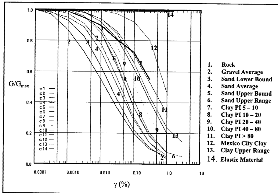
Figure 5. Shear curves
