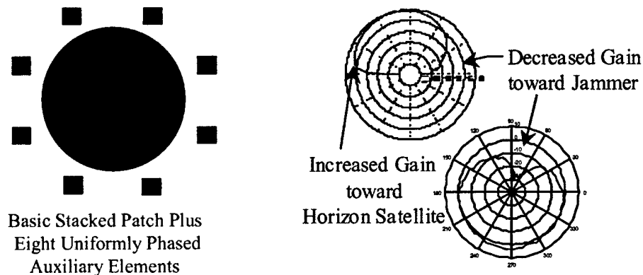
Figure 4. Mode 3 operation
