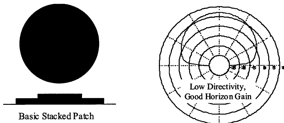
Figure 2. Mode 1 operation
