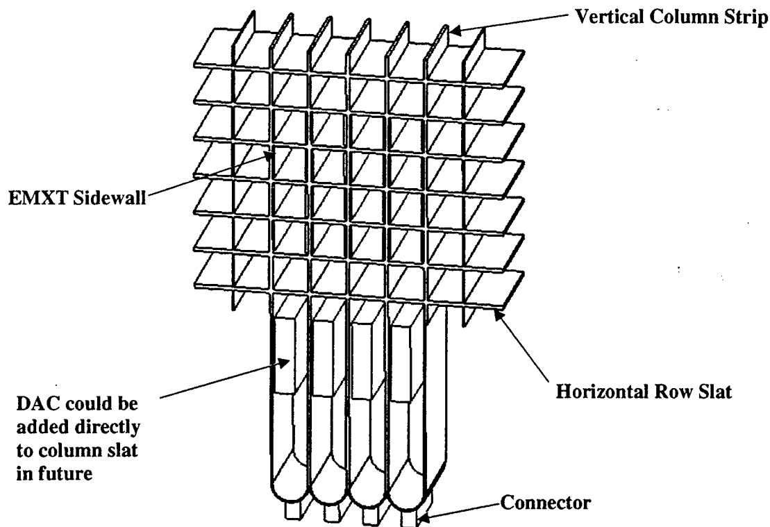
Figure 3-1. Sketch of a 4x4-size array antenna, indicating key elements of a packaging and interconnect approach scalable to larger array.
