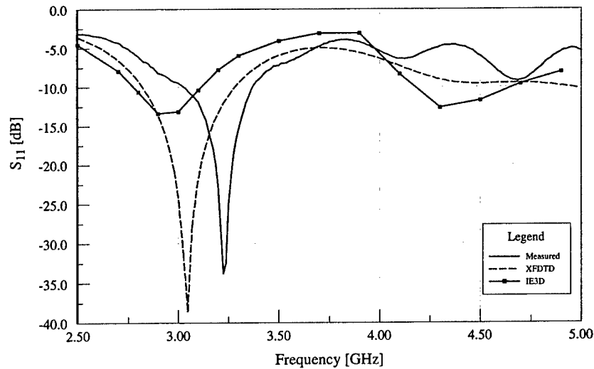
Figure 4: S_{11} Log-magnitude data for the S-band linear bowtie.
