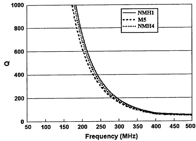
Figure 9. Q Properties of the NMH1, M5 and NMH4 Antenna Configurations.
