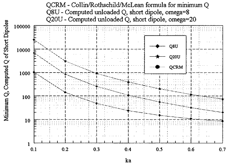
Figure 2. Values of unloaded Q for short dipoles ( \Omega = 8 and 20 ) compared with the values computed for the minimum unloaded Q as a function of antenna size.
