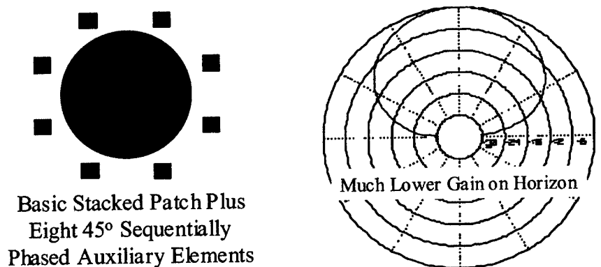
Figure 3. Mode 2 operation
