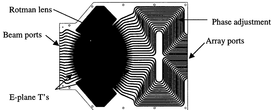
Figure 1. Rotman lens - Shaded areas show signal paths
