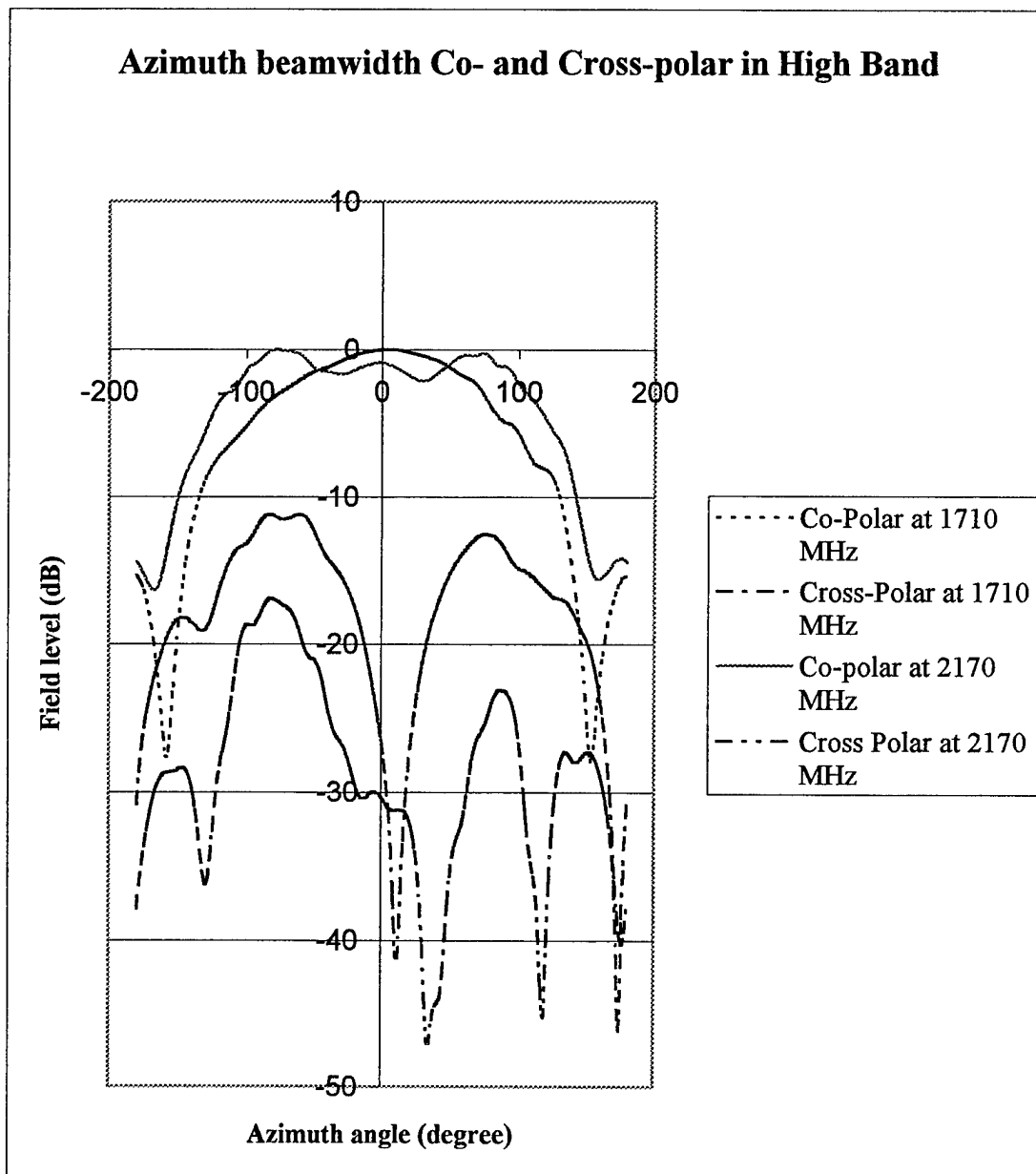
Figure 5. Co- and Cross-Polar Patterns in the frequency band: 1710-2170 MHz
