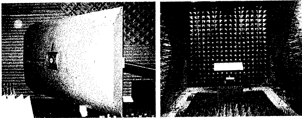
Figure 20. Measurement test facility
