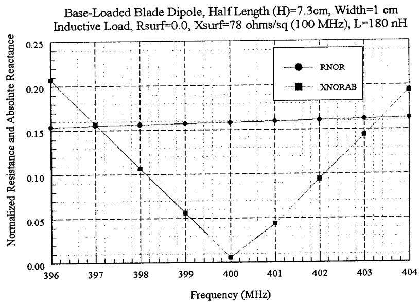
Figure 7. Normalized resistance (RNOR) and absolute value of normalized reactance (XNORAB) computed for a lossless blade dipole using LFMOM code. The short ( ka=0.61 ) dipole is tuned to 400 MHz with a base inductor of 180 nH. The unloaded FWB is 0.016.
