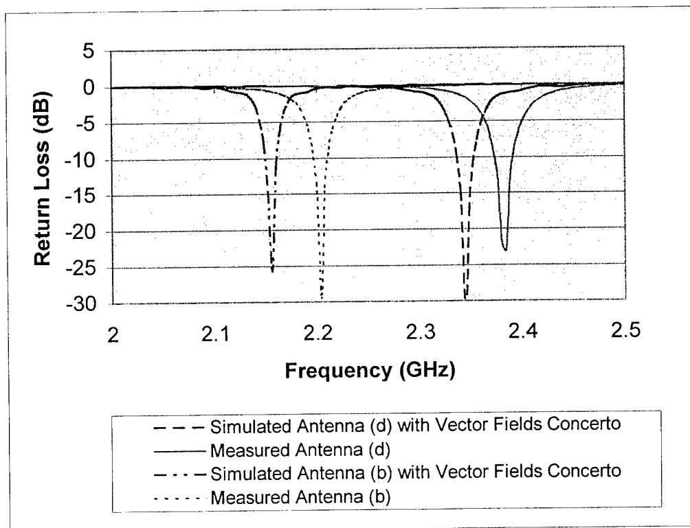
Figure 3. Simulated and measured return lossess of antenna (b) and antenna (d).
