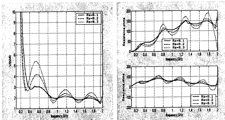
Figure 11. Variation of opening rate ( R_a ) 0.1, 0.2, 0.3 in dielectric-free antenna. D_{sl} = 2 cm, D = 32 cm, broadside beam.
