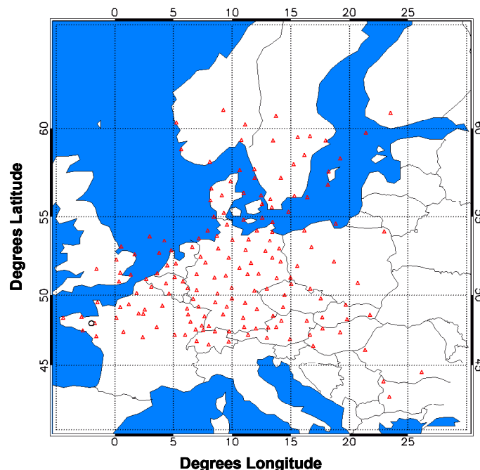
Figure 1. ETEX Sampler Locations Across Europe: Red Open Triangles Correspond to Sampler Locations and the Black Open Circle Corresponds to the Release Location.
