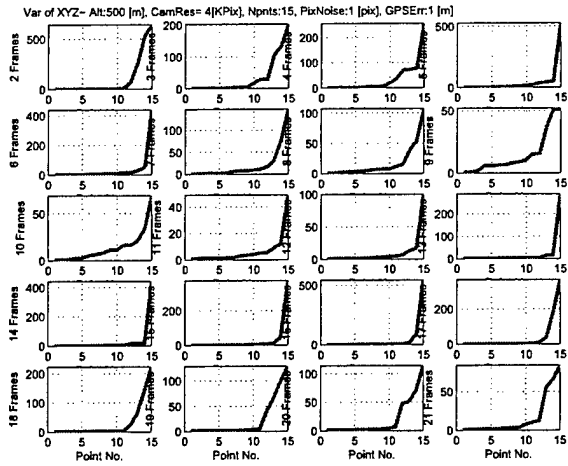
Figure 16: (continued)- Tracking 15 (left) and 30 (right) points with GPS error variance of 1 [m].
