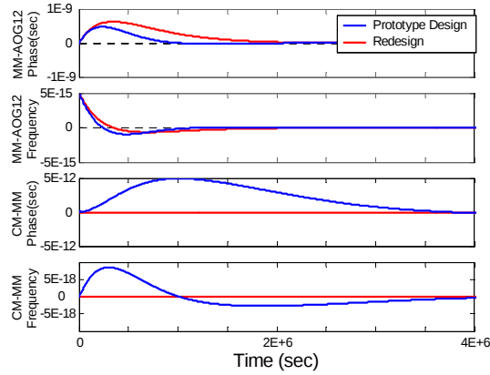
Figure 6. Responses to AOG frequency offset.
