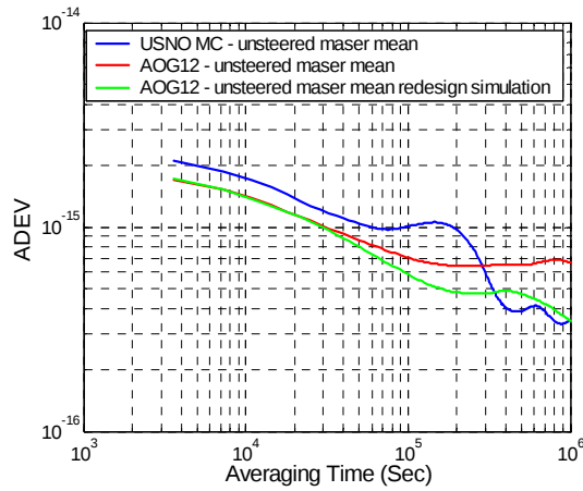
Figure 7. Stability comparison of different designs.
