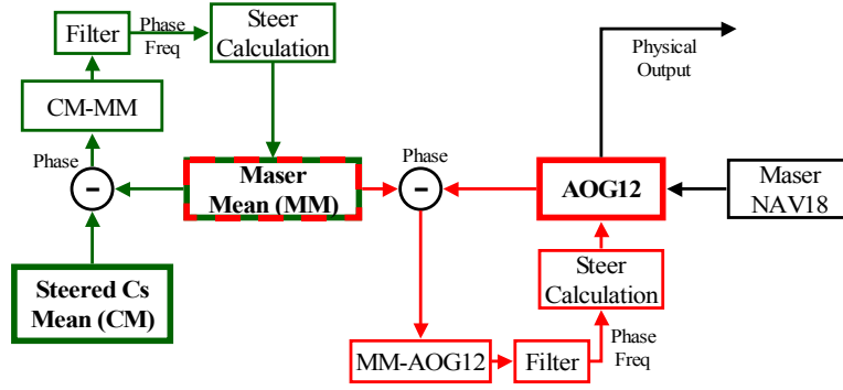
Figure 1. Design Block Diagram.
