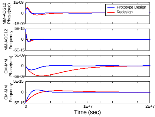
Figure 4. Responses to MM frequency offset.
