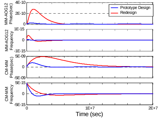
Figure 5. Responses to CM frequency offset.
