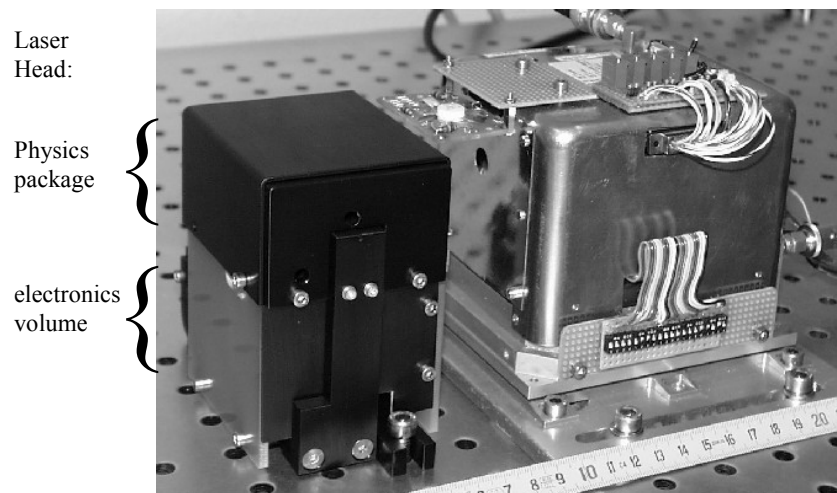
Figure 1. The modular laser-pumped Rb frequency standard. Left: Stabilized laser-head module, including the reference cell. Right: lamp-removed Rb clock unit.
