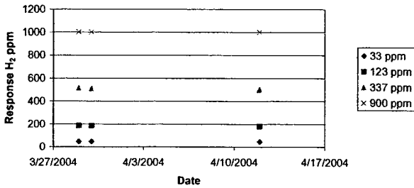
Figure 7. Dräger H 2 Sensor
