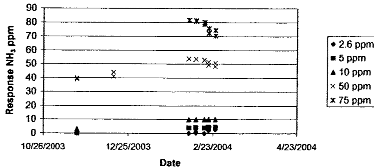
Figure 15. Dräger NH 3 Sensor
