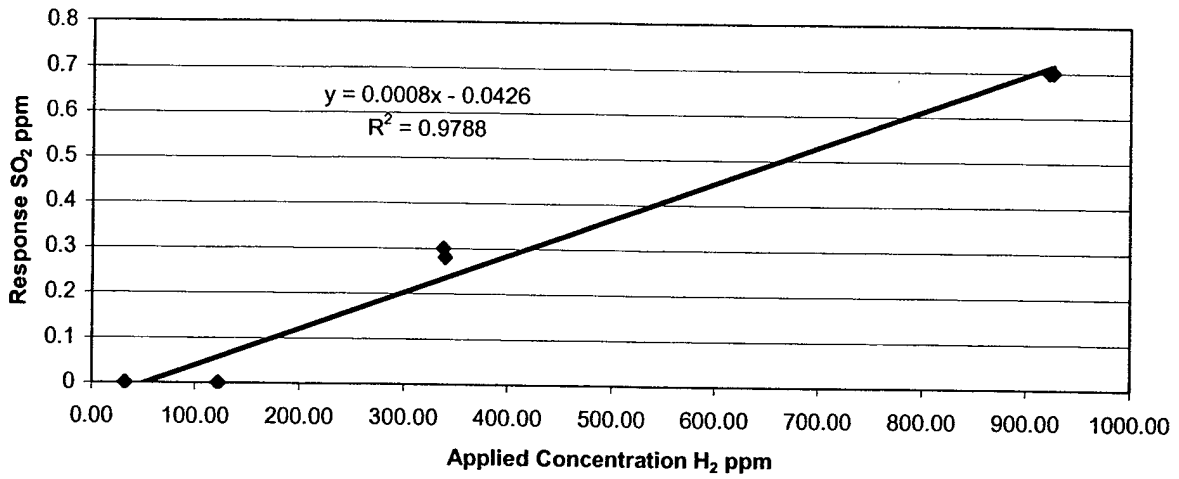
Dräger SO 2 Response to H 2
