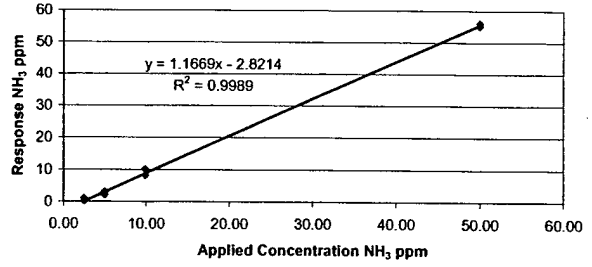
Figure 3. Omni NH 3 Sensor
