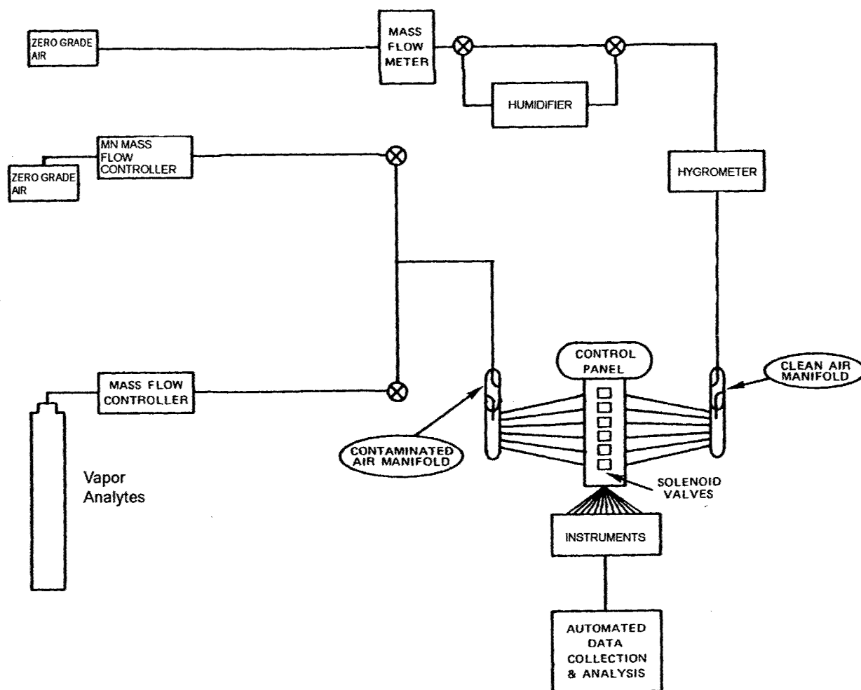
Figure 1. Test manifold designed for the instrument evaluation.
