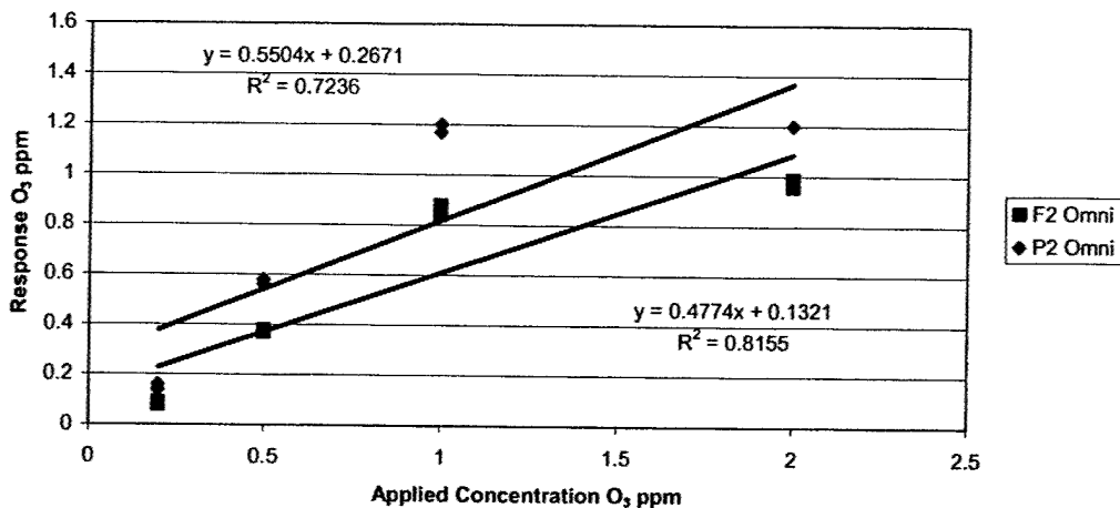
Figure 11. Short Term Data for Two New Omni O 3 Sensors
