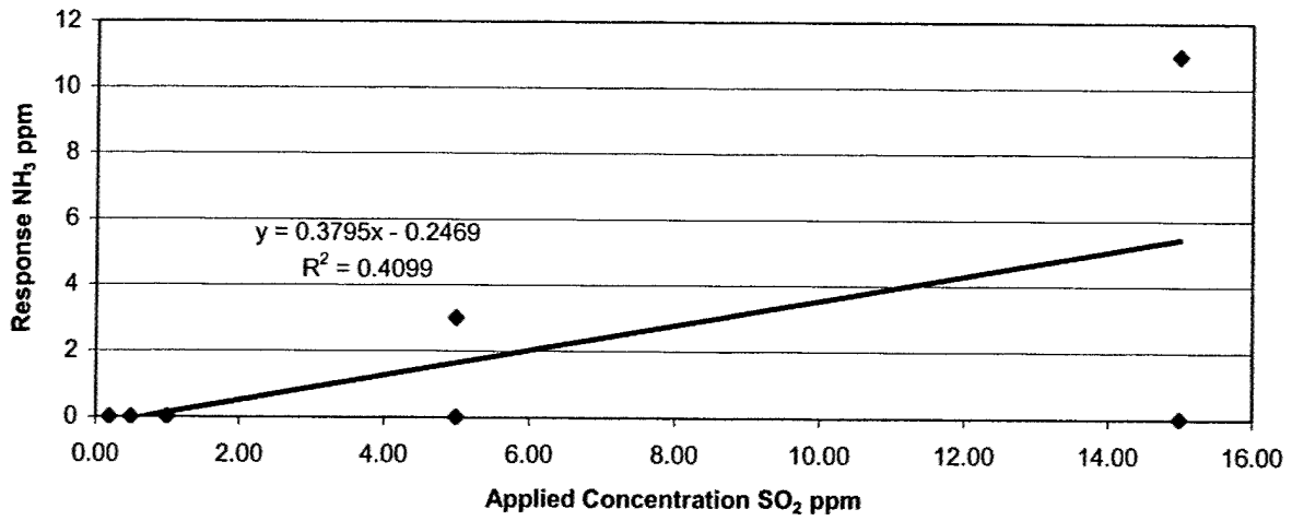
ITX NH 3 Response to SO 2
