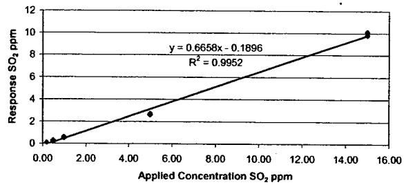
Figure 5. Omni SO 2 Sensor
