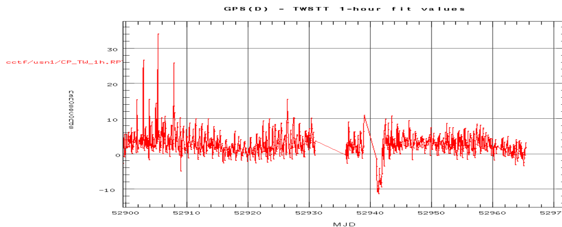
Figure 10. An enlargement of the last 60-days GPS (D) – TWSTT differences to show the improvement because of the program modification.
