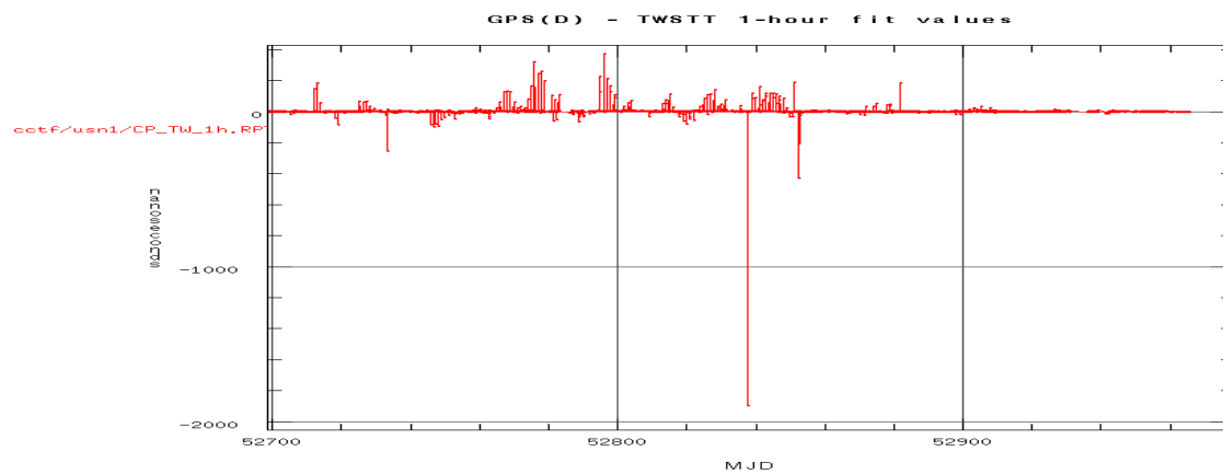
Figure 9. GPS (D) 1-hour linear fit data points differenced from the TWSTT 1-hour linear fitted data points to show how the two processes results differ.
