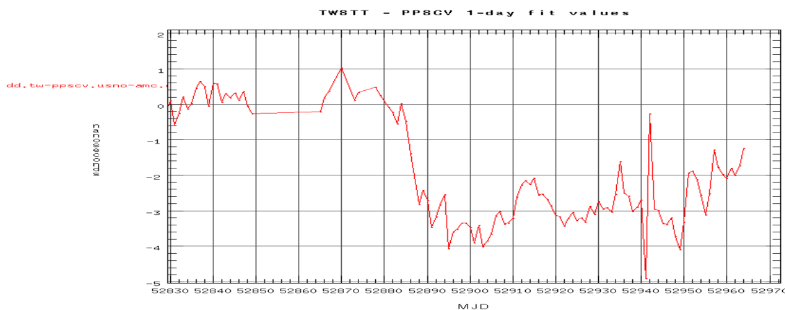
Figure 13. This plot shows the difference between the TWSTT and GPSCV methods between USNO (DC) and USNO (AMC). The GPSCV data uses the PPS receivers at each location common-view differenced. Note the missing data period from MJD 52850 to 52864 and the data step from MJD 52884 to 52886.
