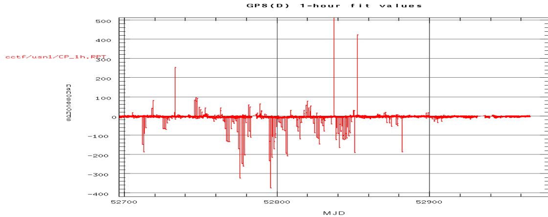
Figure 7. The IGS observational and navigational files for USNO (DC) and USNO (AMC) processed as before, but now linear-fitted over 1-hour periods. The data spikes are due to a program problem that has been fixed. USNO started using the modified program on MJD 52910.
