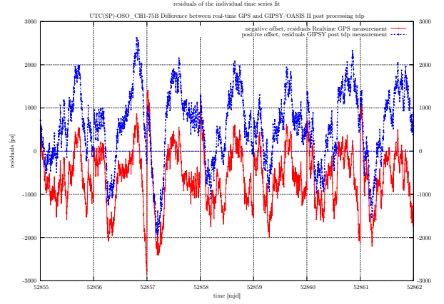
Figure 10: Comparison of the model residuals of RT and GIPSY for the short baseline SPT0-ONSA.
