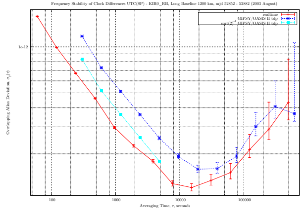
Figure 12: Stability of RT and GIPSY for the long baseline SPT0-KIR0.
