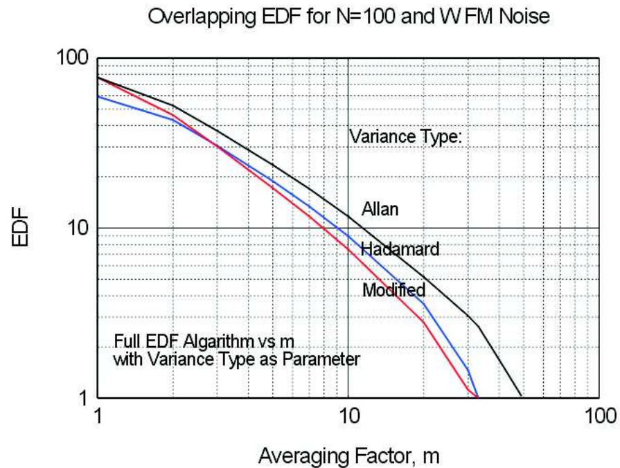
Figure 2. Edf vs. averaging factor for three stability variances: overlapped estimator, white FM, 100 phase samples.
