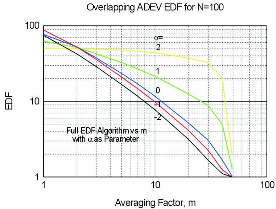
Figure 1. Edf vs. averaging factor with power-law noise type as a parameter: Allan variance, overlapped estimator, 100 phase samples.
