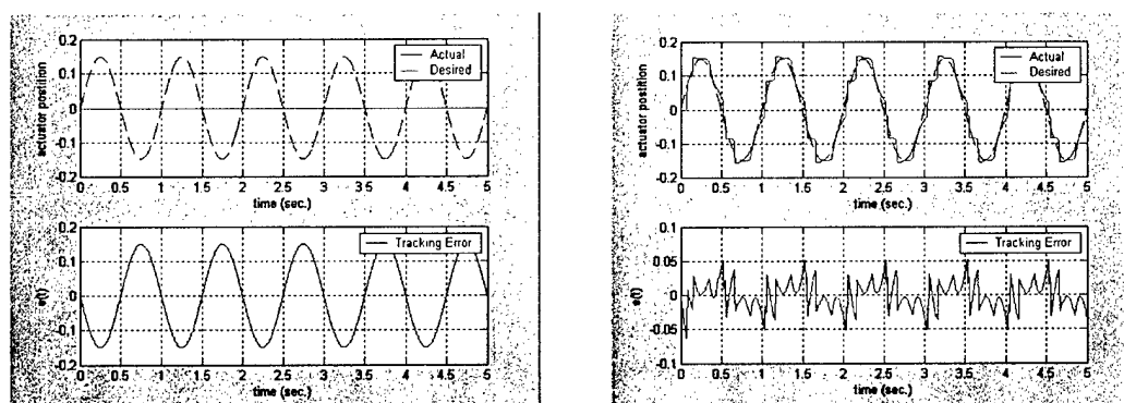
Figure 5-10. Plots Showing No Tracking for Very Small Input without IMPNOR Scheme (left) and Approx. Tracking with IMPNOR Scheme (right)
