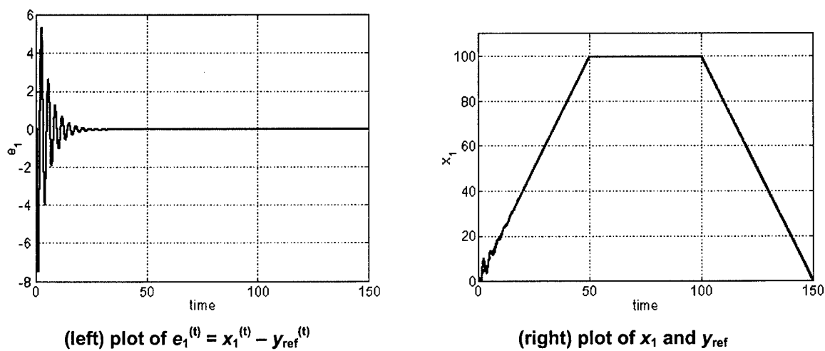
Figure 3-3. e_1 , x_1 , and y_{\text{ref}} in Example 3.3
