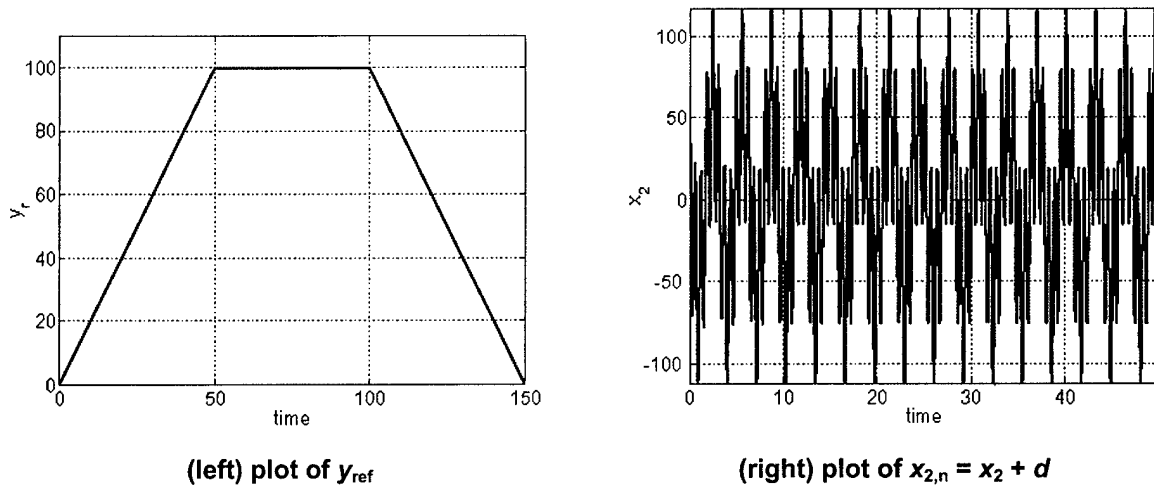
Figure 3-2. y_{\text{ref}} and x_{2,n} in Example 3.3
