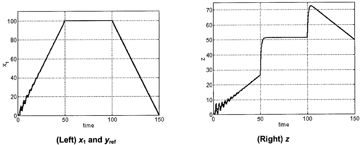
Figure 3-6. x_1 , y_{ref} , and z in Example 3.4
