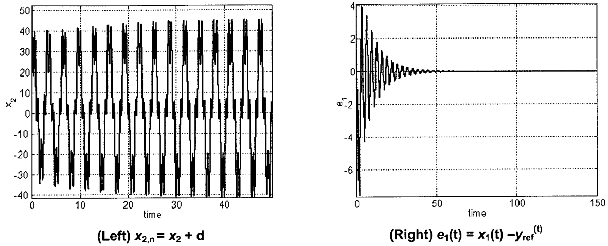
Figure 3-5. x_{2,n} and e_1 in Example 3.4
