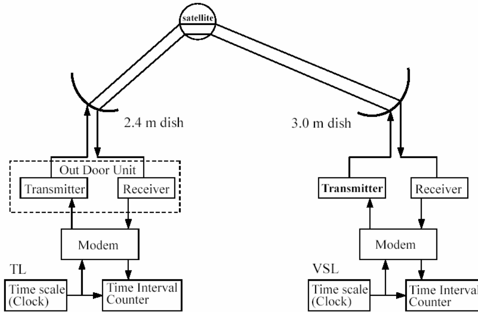
Figure 1(b). Block diagram of the equipment connection for the present TL-VSL link.
