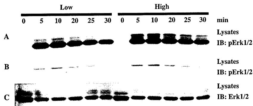
Fig. 4. In high-density cells EGF-dependent activation of Erk1/2 is not suppressed in comparison to the low-density cells. MCF10A cells were treated as described in Fig. 2. Equal amounts of total cellular protein from cell lysates were analyzed by Western blot (IB) for (A) phosphorylated Erk1/2 (pErk1/2). In B, to more effectively examine Erk2, a shorter exposure of (A) was used. In C, Erk1/2 protein expression (Erk1/2) was also assessed by IB analysis. These are representative Western blots from three separate experiments.
