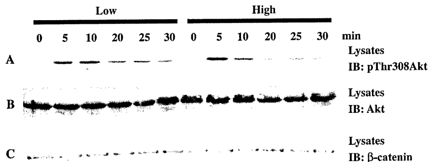
Fig. 7. The EGF-dependent 3-phosphoinositide-dependent kinase-1 phosphorylation (activation) of Akt. MCF10A cells were treated as described in Fig. 2. Equal amounts of total cellular protein from cell lysates were analyzed by Western blot (IB) for (A) phosphothreonine-308 on Akt (pThr308Akt), (B) Akt protein expression (Akt), and (C) \beta -catenin protein expression (used as a loading control in addition to the Akt mass shown in part B). These are representative Western blots from 3 separate experiments. The experiments used for Fig. 3 were stripped and reprobed with the pThr308Akt-specific antibody to generate the data for Fig. 7.
