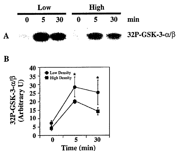
Fig. 8. The EGF-stimulated in vitro kinase activation of Akt is decreased in high-density cells. MCF10A cells were treated as described in Fig. 2. After immunoprecipitating Akt1 from equal amounts of total cellular protein in cell lysates, in vitro phosphorylation of glycogen synthase kinase-3- \alpha/\beta fusion proteins (GSK-3- \alpha/\beta ) was analyzed. In (A), a representative autoradiogram of ^{32}\text{P} -GSK-3- \alpha/\beta is shown. In (B), data from three separate experiments are plotted as a function of GSK phosphorylation. Each point represents the average \pm one standard deviation from phosphoimager analysis. The data are expressed as arbitrary units (U). *designates statistically significant differences between the two densities, P \leq 0.05 by t test.
