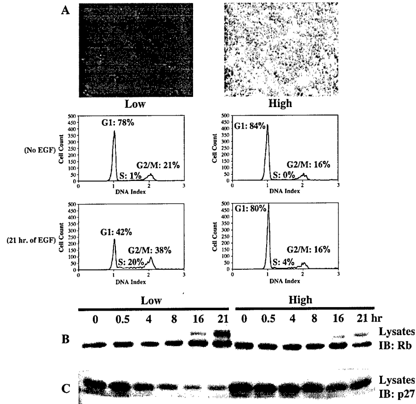
Fig. 1. High-density MCF10A cells do not progress through the cell cycle. MCF10A cells were grown to confluence (high-density), and then half of the cultures were reseeded at 15% confluence (low-density). The cells were placed in growth factor-free media for 18 h and subsequently treated for 21 h (A) or the times indicated (B, C) with 5 ng/ml EGF. (A) Top panels show low- and high-density cell cultures at 100 \times . The cells were processed for cell cycle analysis as described in Materials and methods. DNA histograms were obtained from slides analyzed on an Oncometrics Cyto-Savant automated image cytometer. DNA content was measured according to the Oncometrics protocol using thionine as the DNA stain. The calculated sum optical density (DNA index) was plotted vs. frequency (cell count). Middle panels show the cell cycle profiles of low- and high-density cells under growth factor starved conditions. Lower panels show the cell cycle profiles of low- and high-density cells after 21 h of treatment with 5 ng/ml of EGF. (B, C) analyzes equal amounts of total cellular protein from cell lysates by Western blot (IB) for (B) phosphorylated retinoblastoma protein (Rb-slower migrating band) or hypophosphorylated Rb (faster migrating band) and (C) p27 protein expression (p27).
