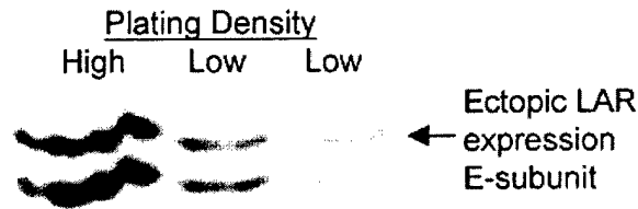
Figure 4 Density-dependent regulation of ectopically expressed LAR
