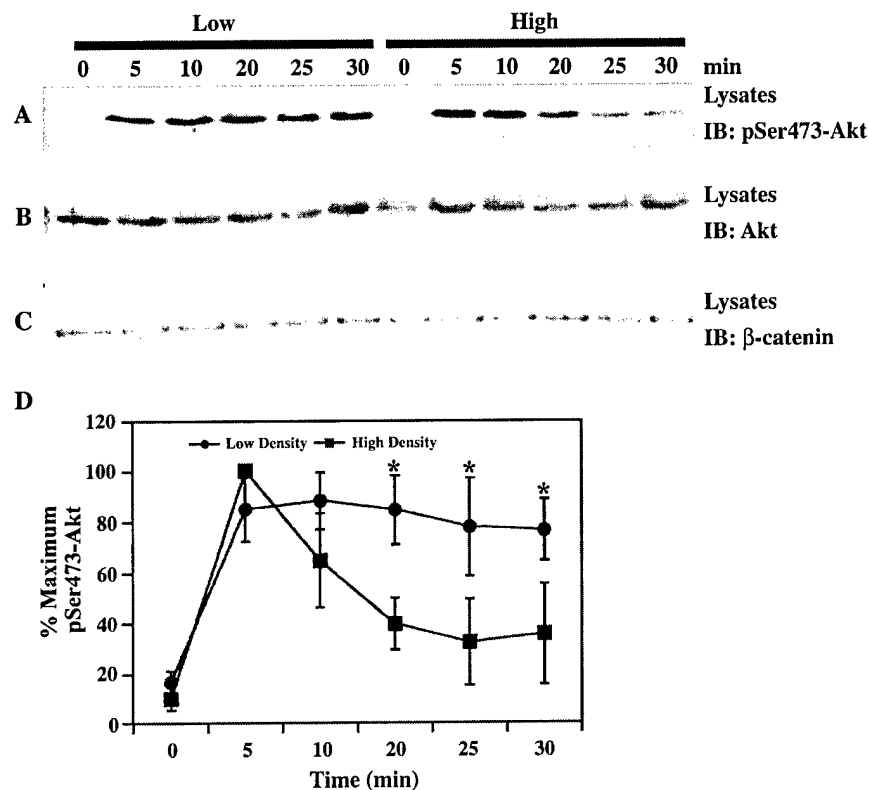
Fig. 3. EGF-dependent Akt activation is transient in high-density cells and sustained in low-density cells. MCF10A cells were treated as described in Fig. 2. Equal amounts of total cellular protein from cell lysates were analyzed by Western blot (IB) for (A) phosphoserine-473 on Akt (pSer473-Akt) and (B) Akt protein expression (Akt) under high- and low-density conditions. In C, \beta -catenin is used as a loading control (in addition to the Akt protein mass shown in part B). In D, data are plotted as percentage of maximum serine-473-Akt phosphorylation as a function of time (see Materials and methods). Each point represents the average \pm one standard deviation from densitometry scans of three separate experiments. *designates statistically significant differences between the two densities, P \leq 0.05 by t test.
