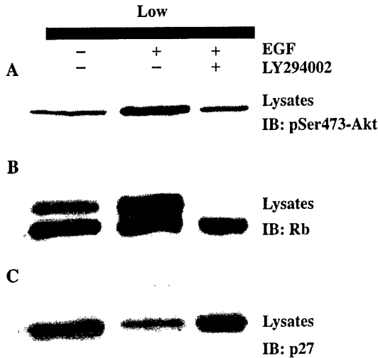
Fig. 10. Inhibition of PI3 kinase mediated Akt activation blocks cell cycle progression in low-density cells. Low-density cells were treated for 21 h with or without 5 ng/ml of EGF. After an initial 30 min of EGF treatment, the cells were further treated \pm 30 \mu\text{M} LY294002. Equal amounts of total cellular protein from cell lysates were separated by SDS-PAGE, and Western blot (IB) analysis of (A) phosphoserine-473 on Akt (pSer473-Akt), (B) retinoblastoma protein phosphorylation (Rb), and (C) p27 protein expression (p27) are shown.
