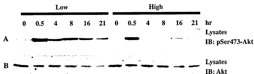
Fig. 9. EGF-dependent Akt activation remains suppressed in high-density cells during long-term EGF stimulation. MCF10A cells were treated as described in Fig. 1. Equal amounts of total cellular protein from cell lysates were analyzed by Western blot (IB) analysis for (A) phosphoserine-473 on Akt (pSer473-Akt) and (B) Akt mass (Akt) (Part A was overexposed to show pSer473-Akt in the high-density cells).
