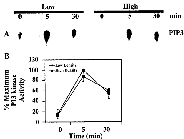
Fig. 6. The EGF-dependent Gab1-associated in vitro PI3 kinase activation is similar in low- and high-density cells. MCF10A cells were treated as described in Fig. 2. Equal amounts of total cellular protein from cell lysates were immunoprecipitated (IP) with anti-Gab1 antibody (Gab1) and analyzed for associated PI3 kinase activation as described in Materials and methods. In A, a representative autoradiogram of ^{32}\text{P} -phosphatidylinositol-3-phosphate (PIP3) is shown. In B, data from three separate experiments are plotted as a function of maximum PI3-kinase activity (see Materials and methods). Each point represents the average \pm one standard deviation from phosphoimager analysis of three separate experiments.
