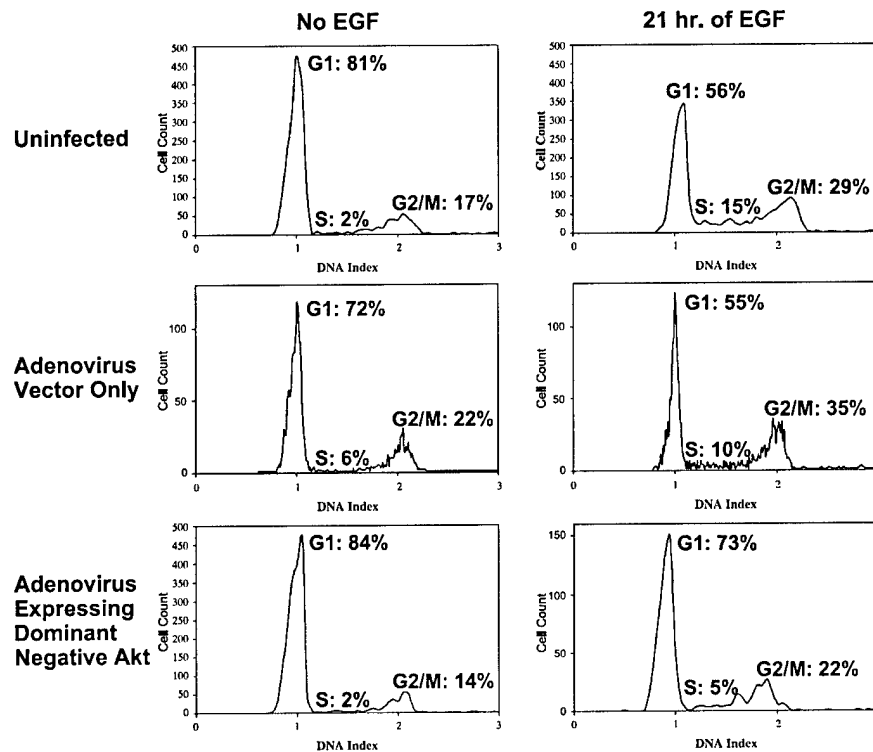
Fig. 11. Adenovirus mediated expression of dominant-negative Akt prevents cell cycle progression in low-density cells. Low-density cells were infected with adenovirus containing dominant-negative Akt or control adenoviral DNA. The infected cells as well as the uninfected control cells were treated \pm 5 \text{ ng/ml} EGF for 21 h and processed for cell cycle analysis as described in Materials and methods. DNA histograms were obtained from slides analyzed on an Oncometrics Cyto-Savant automated image cytometer. DNA content was measured according to the Oncometrics protocol using thionine as the DNA stain. The calculated sum optical density (DNA index) was plotted vs. frequency (cell count).
