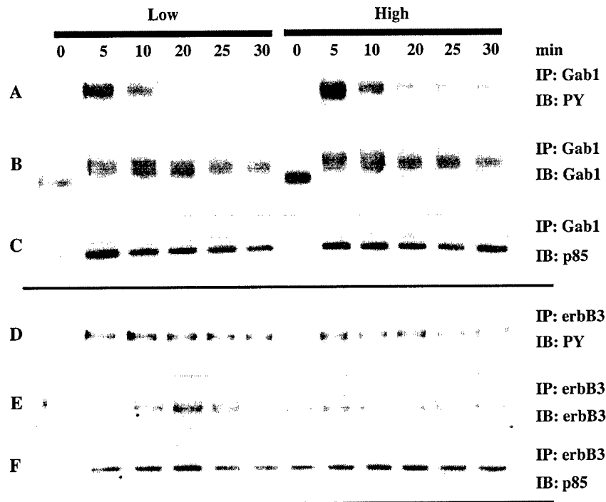
Fig. 5. EGF-dependent tyrosine phosphorylation of Gab1 and erbB3, and their association with p85 subunit of PI3 kinase are comparable in high- and low-density cells. MCF10A cells were treated as described in Fig. 2. Equal amounts of total cellular protein from cell lysates were immunoprecipitated (IP) with (A, B, C) anti-Gab1 (Gab1) or (D, E, F) anti-erbB3 antibodies. Western blots (IB) were then probed with antibodies to (A, D) phosphotyrosine (PY), (B) Gab1 (Gab1), (C, F) p85 subunit of PI3 kinase (p85), and (E) erbB3 (erbB3).
