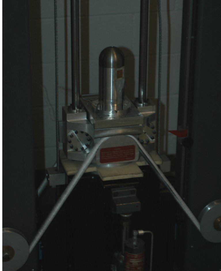
Figure 13. Imager round mounted to shock table.
