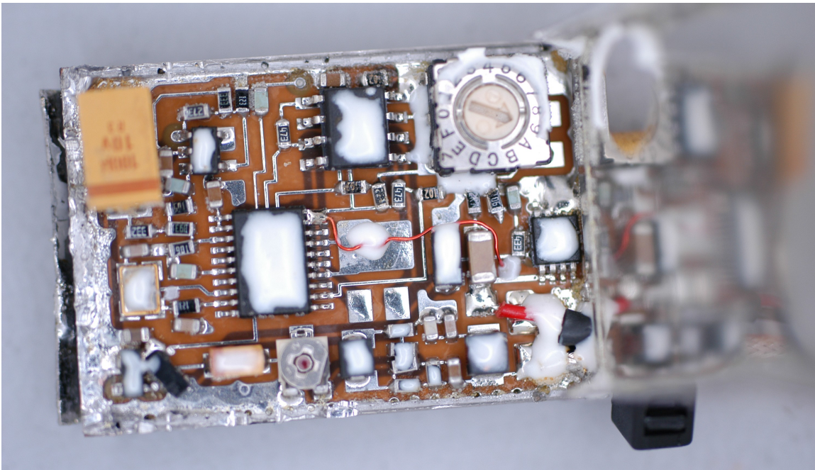
Figure 10. Southern California Microwave VNTX transmitter.
