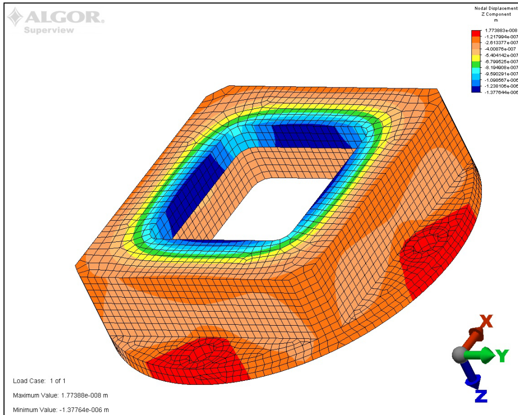
Figure 18. Displacement of revised mounting box.
