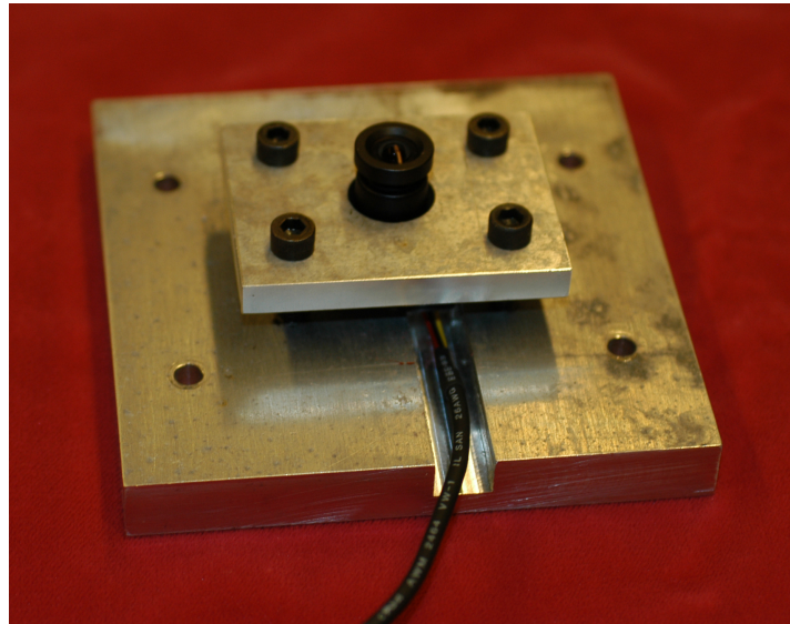
Figure 5. Camera mounted in shock fixture.
