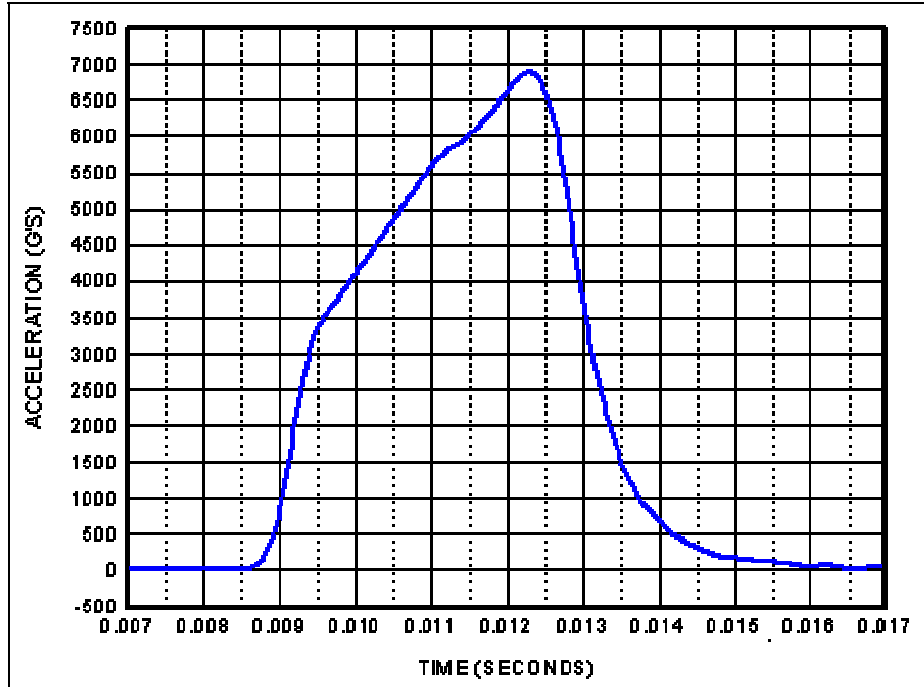
Figure 9. BDM nominal acceleration.
