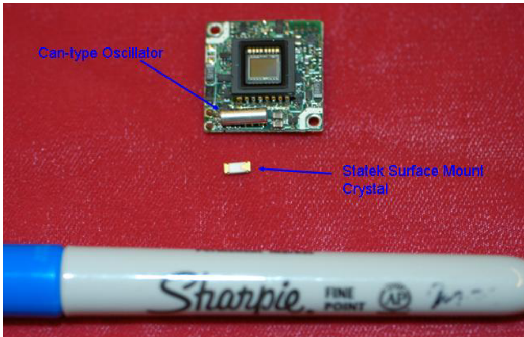
Figure 17. PC72XS camera circuit board with Statek crystal.
