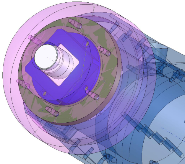
Figure 8. Solid model showing the camera installed in the imager warhead.
