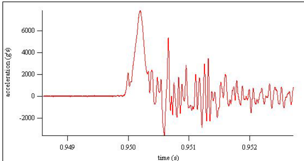
Figure 14. Recorded shock pulse during test of video imager.
