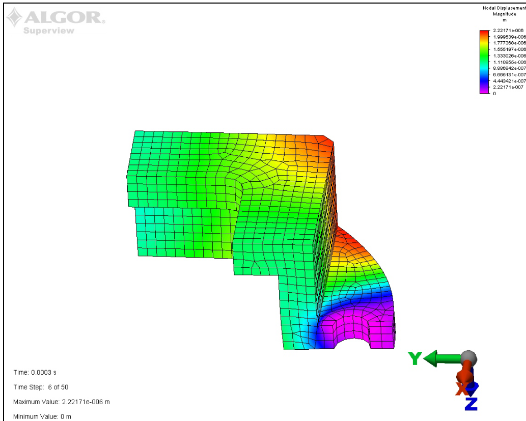
Figure 19. Displacement of the camera mounting box in dynamic analysis.
