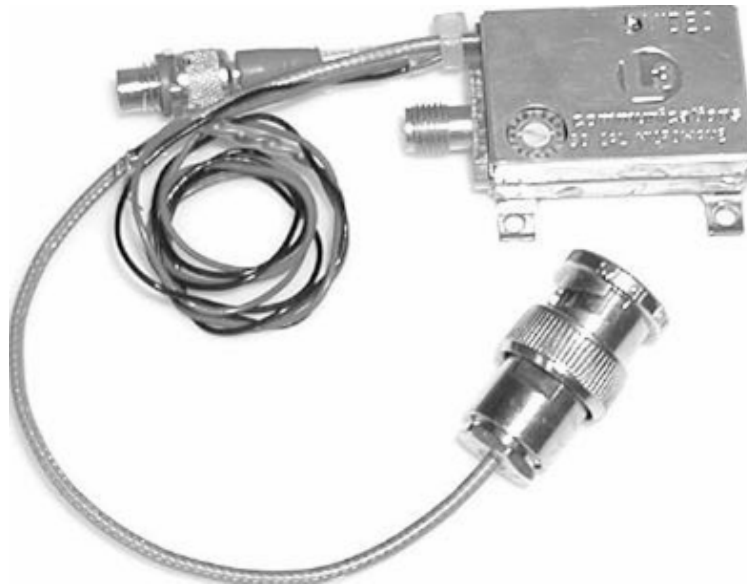
Figure 1. VNTX transmitter.
