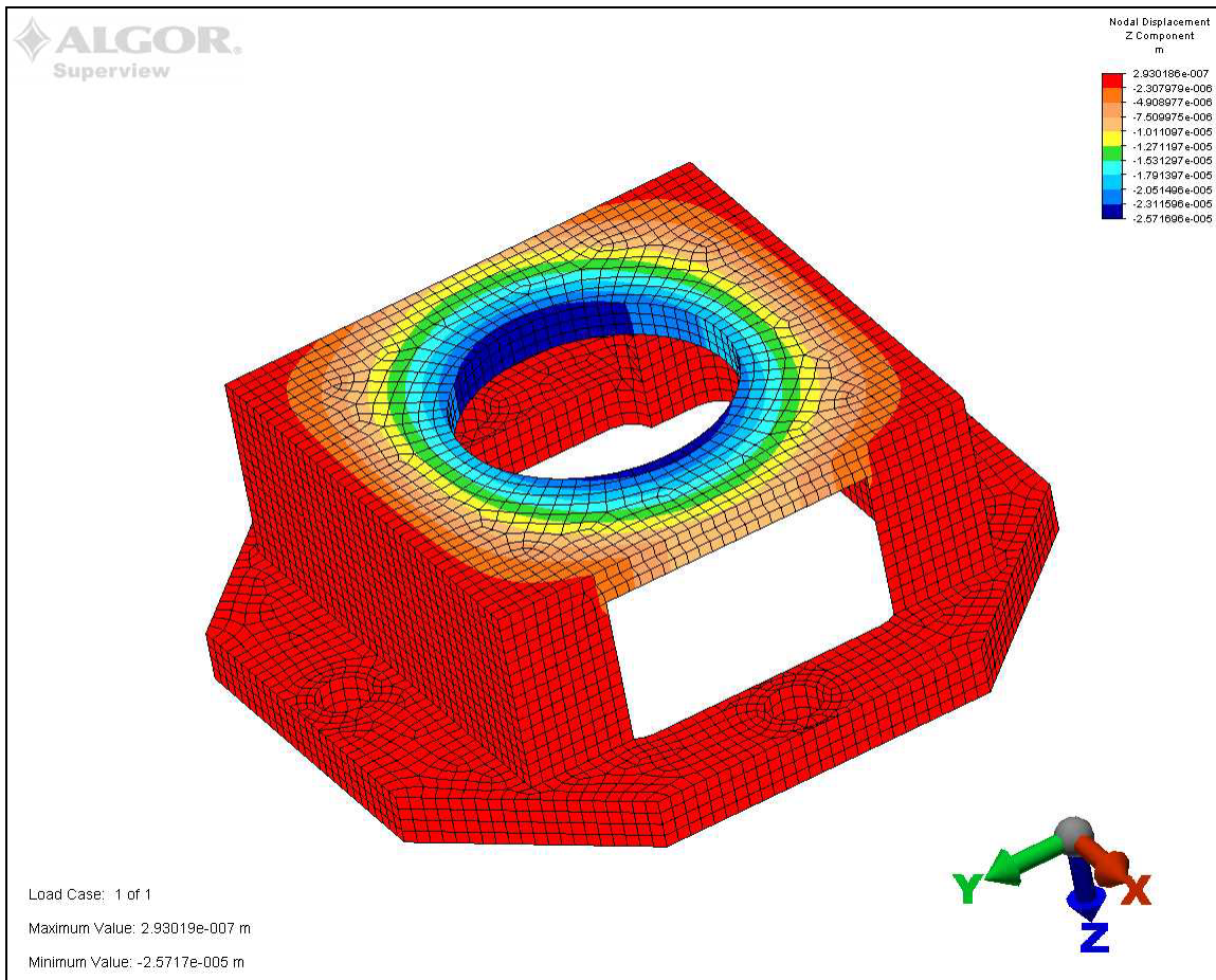
Figure 16. Displacement graph of the mounting box from FEA.
