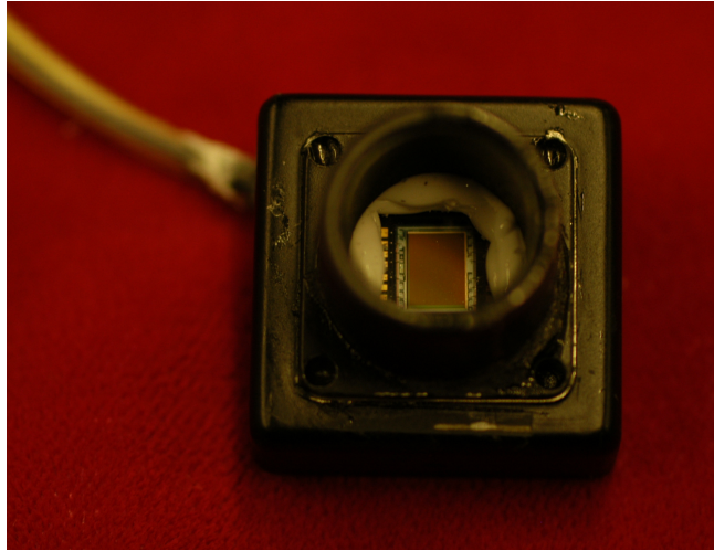
Figure 11. Encapsulated camera showing the RTV sealant around the CCD.
