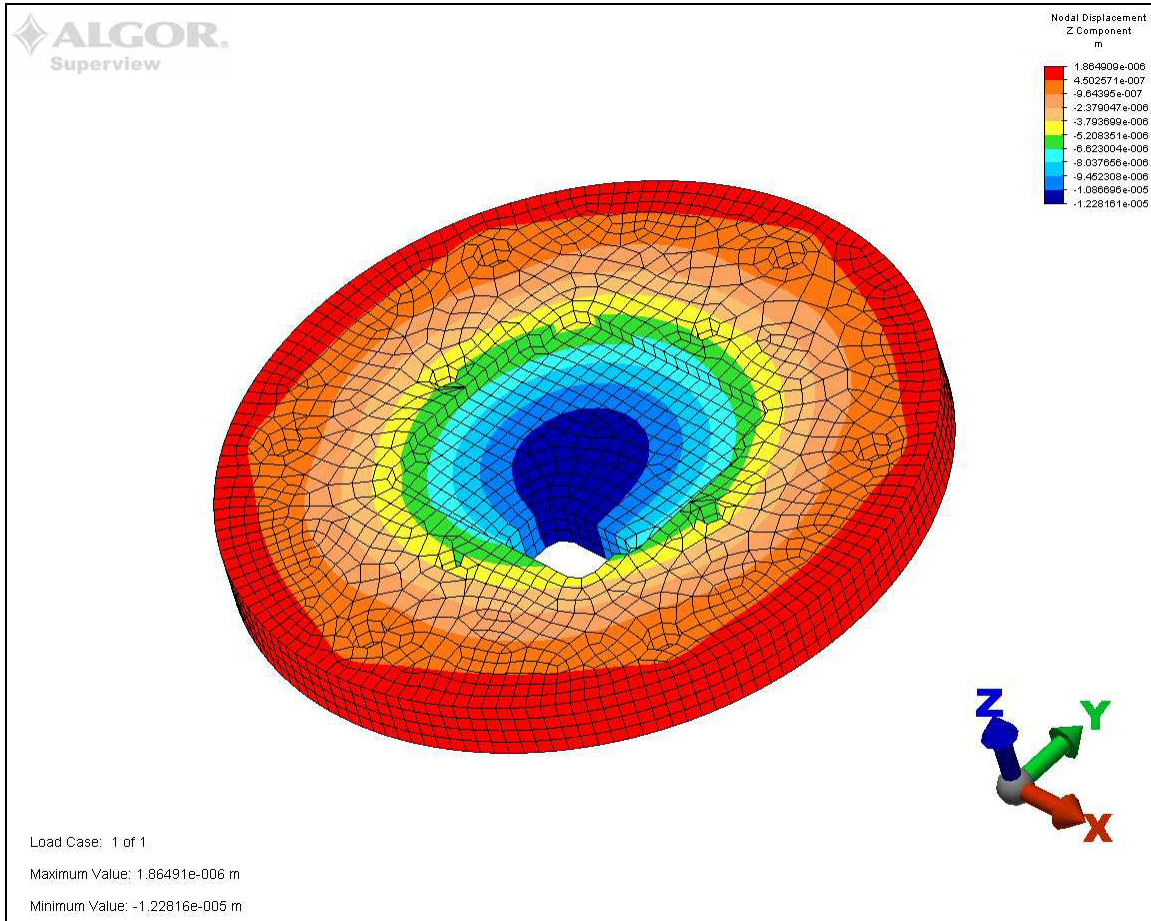
Figure 15. Displacement graph of the camera mounting plate from FEA.
