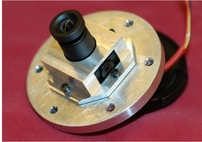
Figure 7. The PC182XS camera mounted in the camera mounting plate and mounting box.
