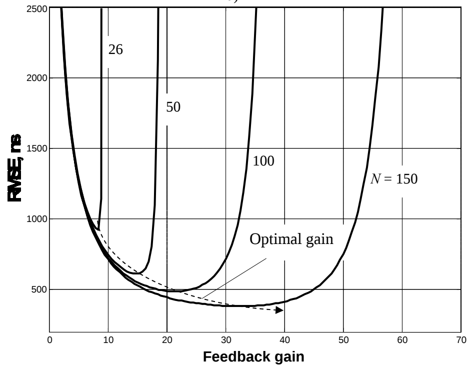
Figure 4. RMSE of the steered crystal clock as function of the feedback gain for several numbers N of the points in the filter kernel: a) CK FIR, b) LK FIR.
