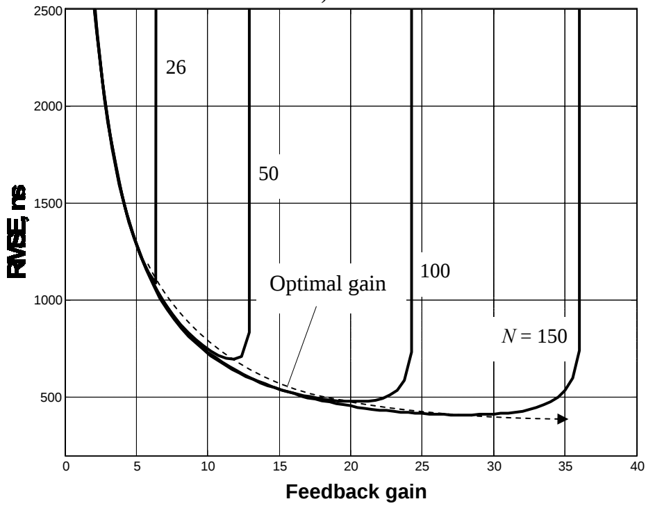
Figure 3. RMSE of the steered crystal clock as function of the feedback gain for several numbers N of the points in the filter transient: a) 2D Kalman, b) 3D Kalman.
