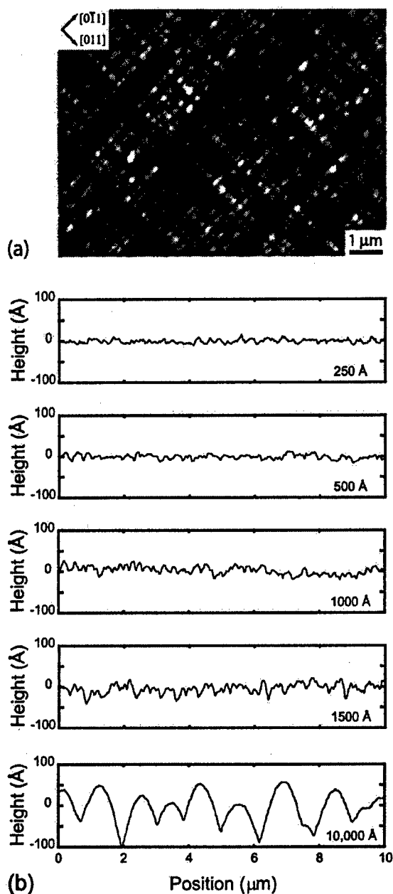
FIG. 3. AFM results of cross-hatch surface morphology in \text{In}_{0.25}\text{Ga}_{0.75}\text{As}/\text{GaAs} ( \epsilon_m = 1.8\% ) films. (a) Plan view surface cross-hatch topography for a typical 70% relaxed h = 1000 \text{ Å} thick film. (b) Surface height profile along the [011] line direction of h = 250, 500, 1000, 1500 , and 10\,000 \text{ Å} films. Note the increasing height variation and the formation of hillocks and valleys with increasing thickness.
