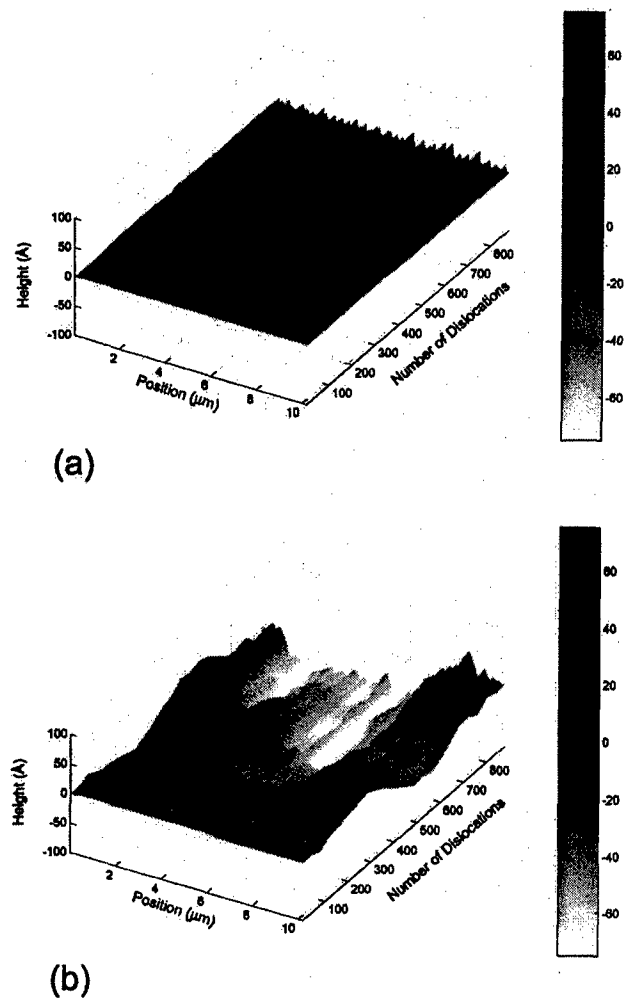
FIG. 8. Surface height profile evolution with increasing strain relaxation. (a) SSO case where there is little variation in the surface height profile. (b) SSE case where there are large variations in surface height profile. The modeled film composition \text{In}_{0.25}\text{Ga}_{0.75}\text{As} corresponds to G=2.90 GPa, \nu=0.32 , and \epsilon_m=1.8\% ; film thickness h=1000 Å.
