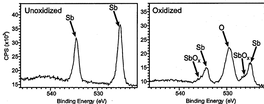
FIG. 7. XPS spectra of the \text{AlAs}_{0.8}\text{Sb}_{0.2} interlayer before and after oxidation. The unoxidized spectrum shows the Sb in the AlAsSb interlayer. After lateral wet oxidation, the spectrum peaks corresponded to the remaining Sb that was 15% oxidized and the oxygen in the \text{AlO}_x interlayer.
