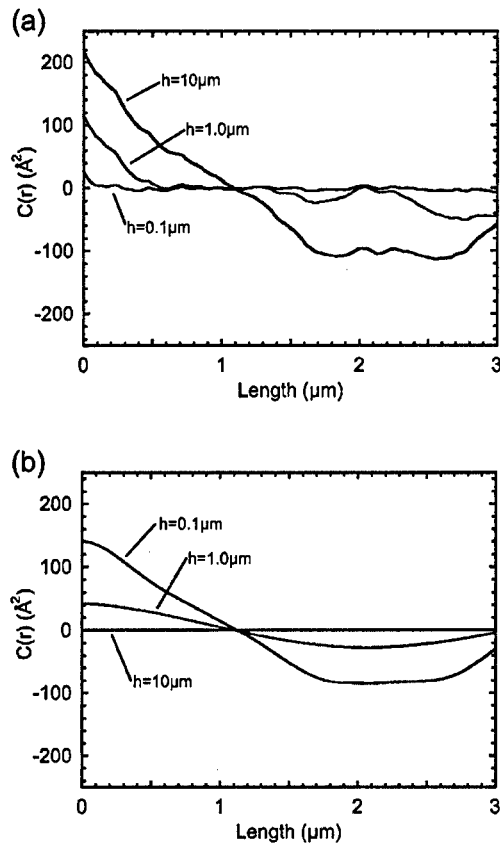
FIG. 7. Height-height correlation functions C(r) for surface profiles in the model with randomly nucleated dislocation for SSO (a) and SSE (b) cases for different film thicknesses. The data correspond to a fully relaxed \text{In}_{0.25}\text{Ga}_{0.75}\text{As} layer with \nu=0.32 , and \epsilon_m=1.8\% .
